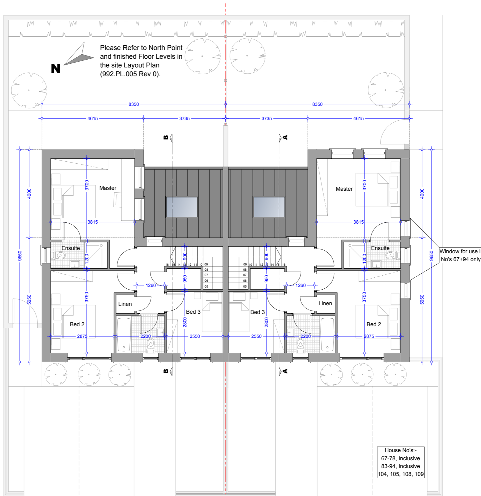
First Floor Plan - House Type A - 3Bed Semi (Mid Street) Area = 53.21 m2 / 572.70 Sqf
