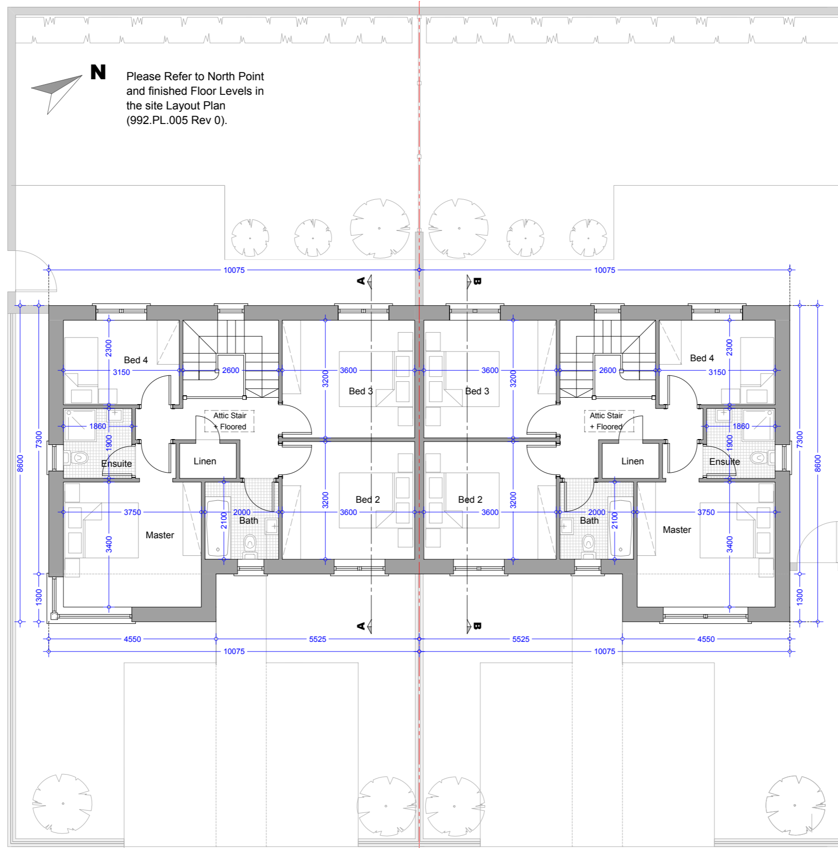
First Floor Plan - House Type B - 4Bed Semi (End of Street) Area = 66.95m 2 / 720.64 Sqf
