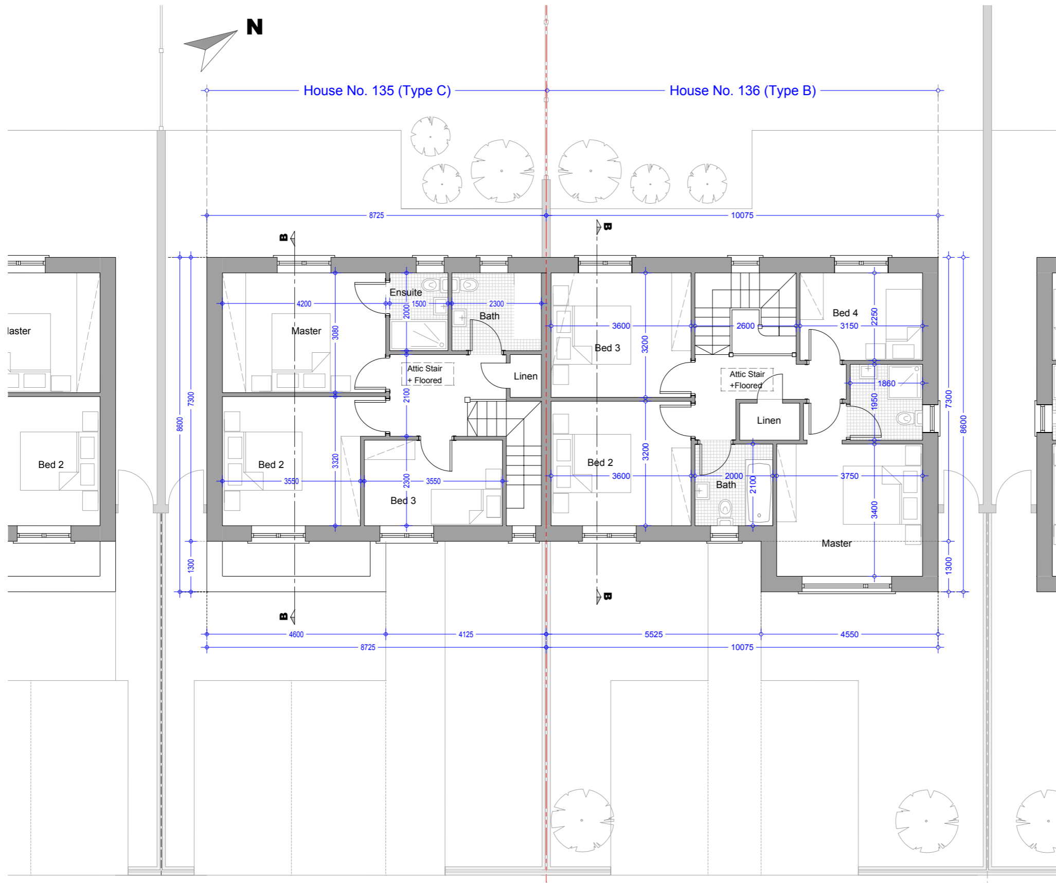
First Floor Plan - House Type C (Mid Street) Area = 53.29 m 2 / 573.60 Sqf
