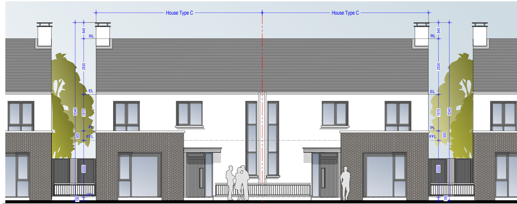
Front Elevation - House Type C (Mid Street)
