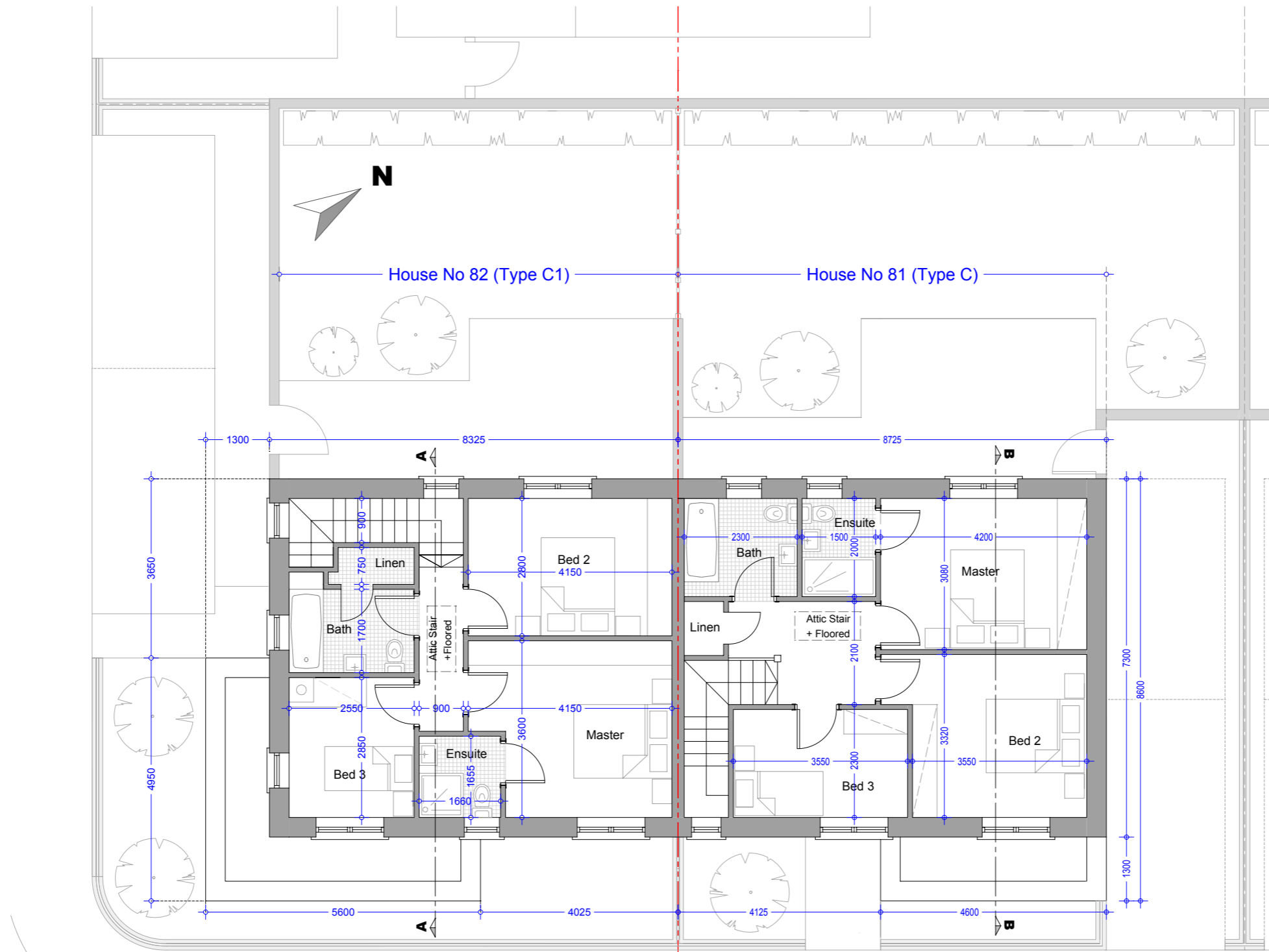
First Floor Plan - House C1 - 3Bed Semi Area = 50.8 m 2 / 546.80 sqf
