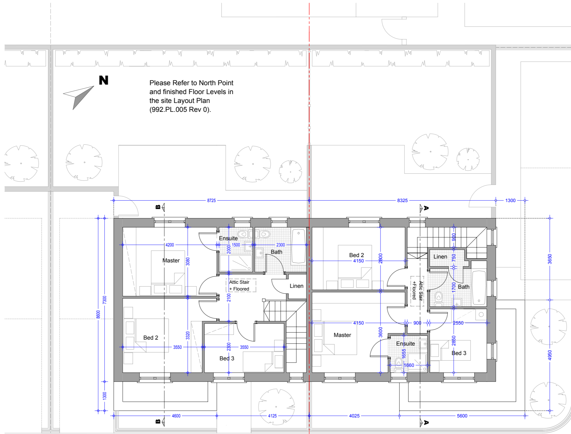
First Floor Plan - House Type C - 3Bed (Mid Street) Area = 53.29 m2 / 573.60 Sqf
