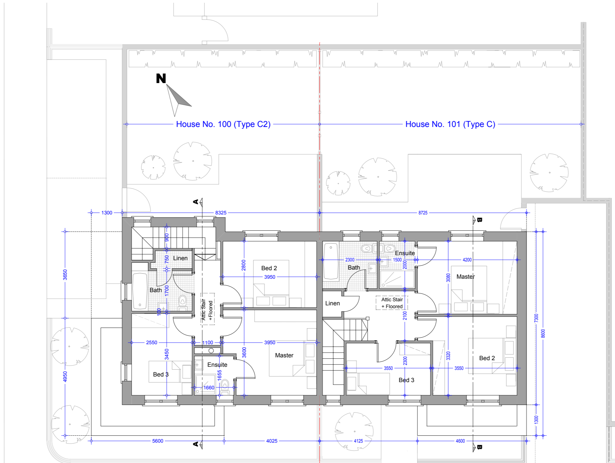
First Floor Plan - House Type C - 3Bed (Mid Street) Area = 53.29 m2 / 573.60 Sqf
