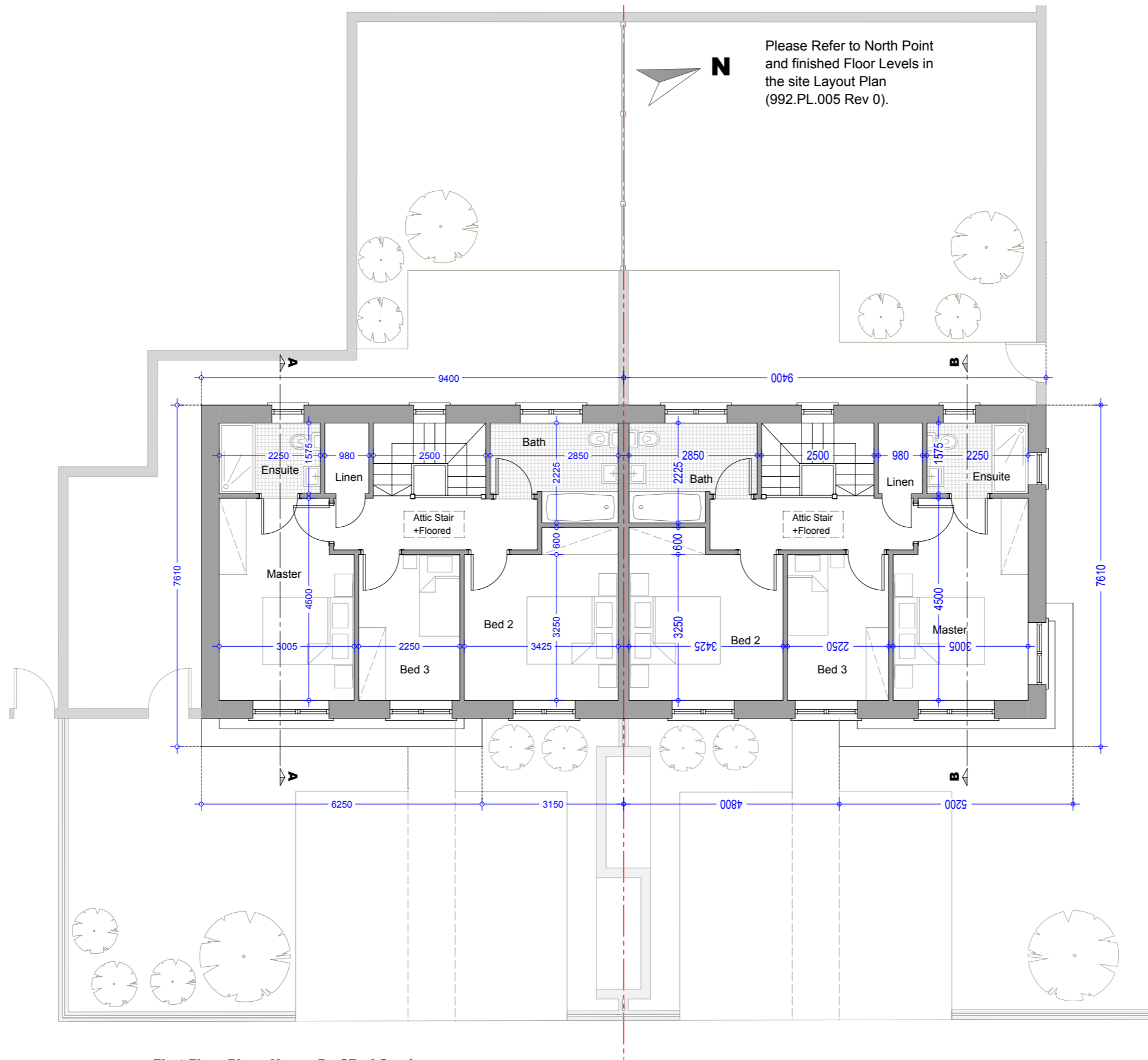
First Floor Plan - House D1 - 3Bed Semi Area = 54.83 m2 / 590.18 sqf
