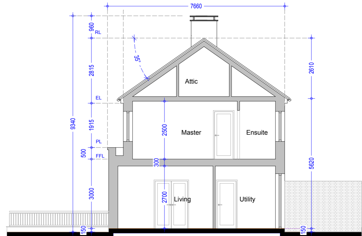
Section AA - House Type D1 (Detached)
