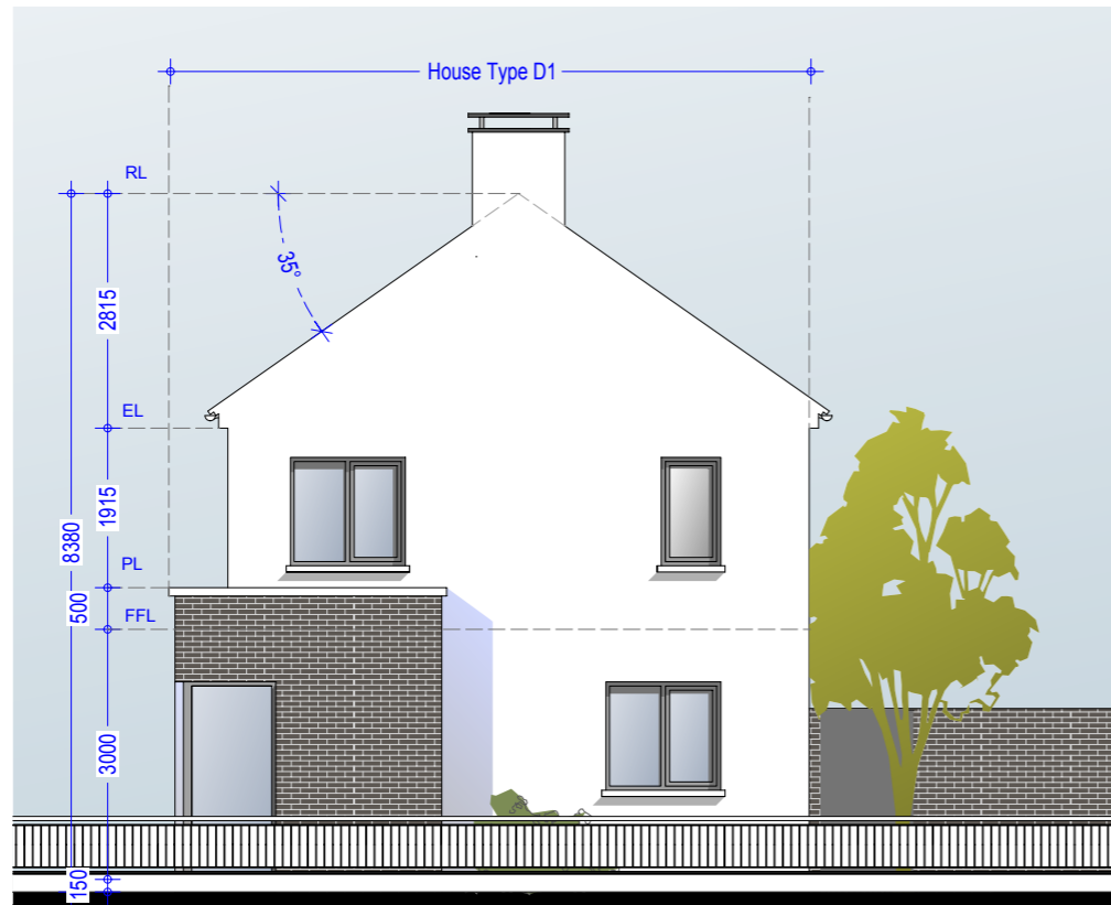
Side Elevation 02 - House Type D1 (Detached)
