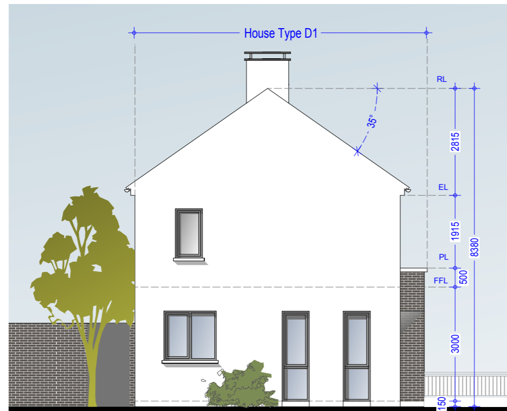
Side Elevation 01 - House Type D1 (Detached)
