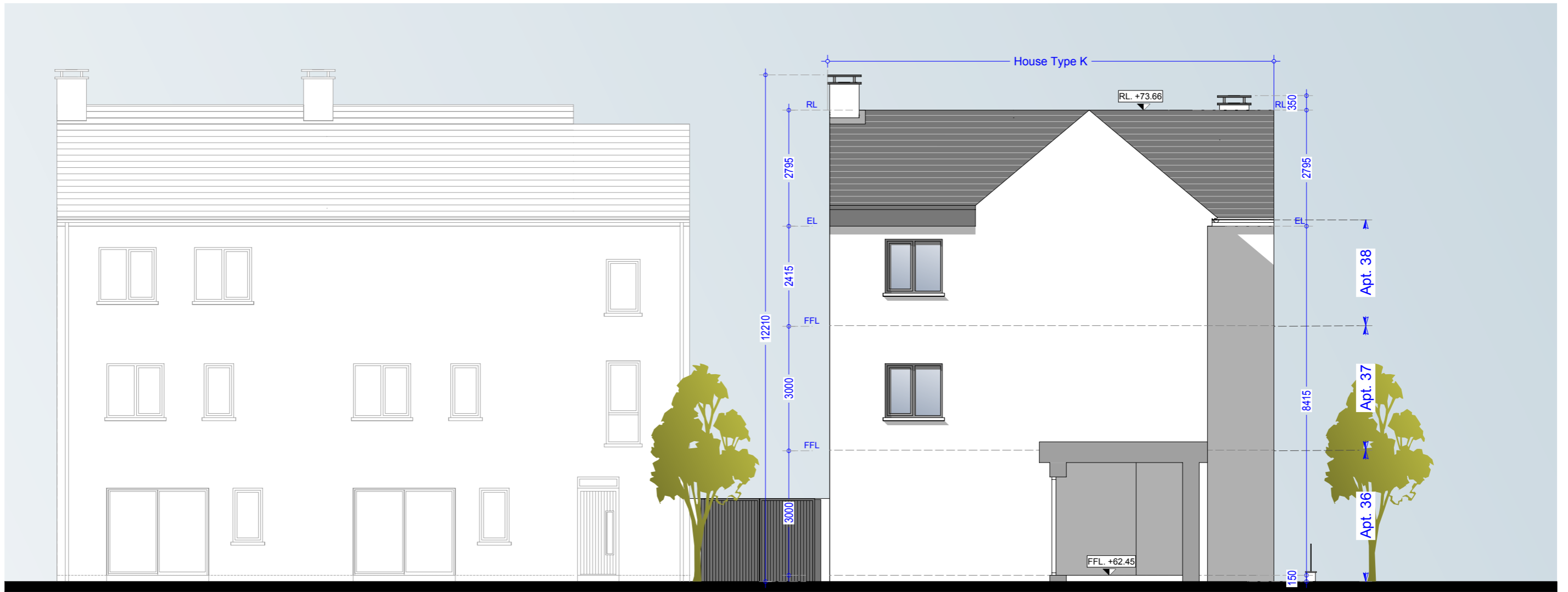
Rear (South West) Elevation & Section BB - 1Bed Apartments No. 36 to 38
