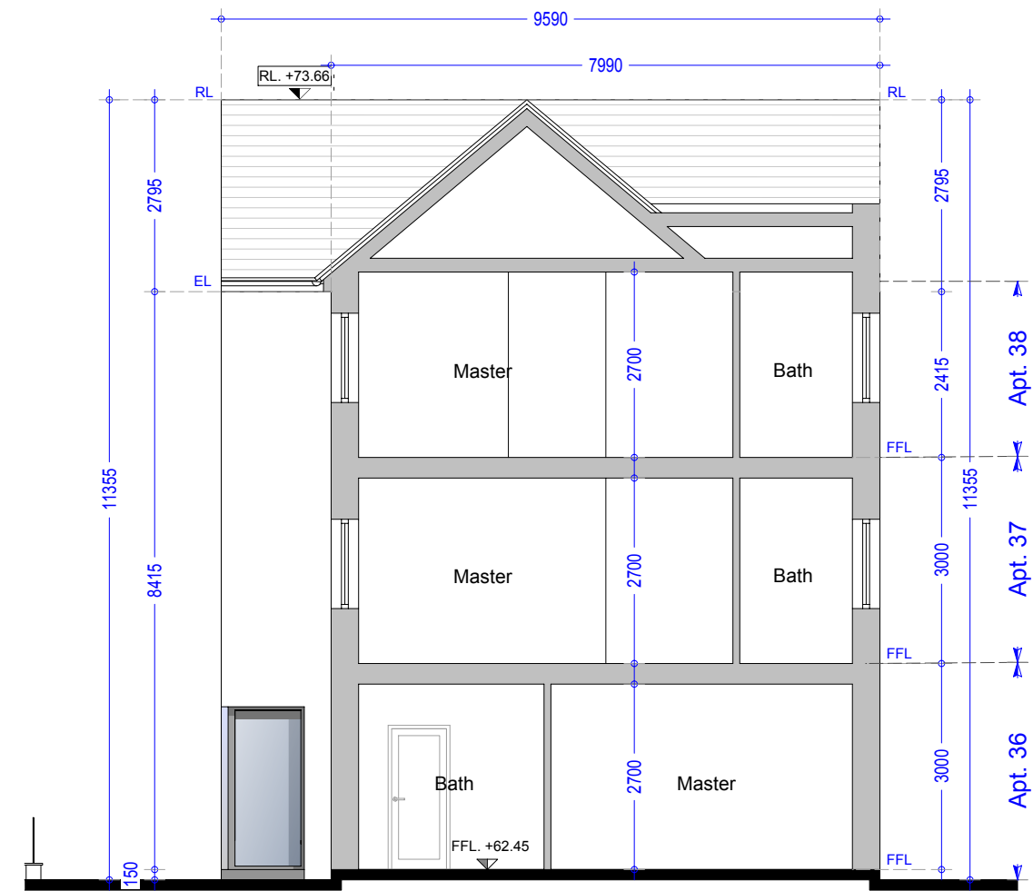
Section AA - 1Bed Apartments No. 36 to 38
