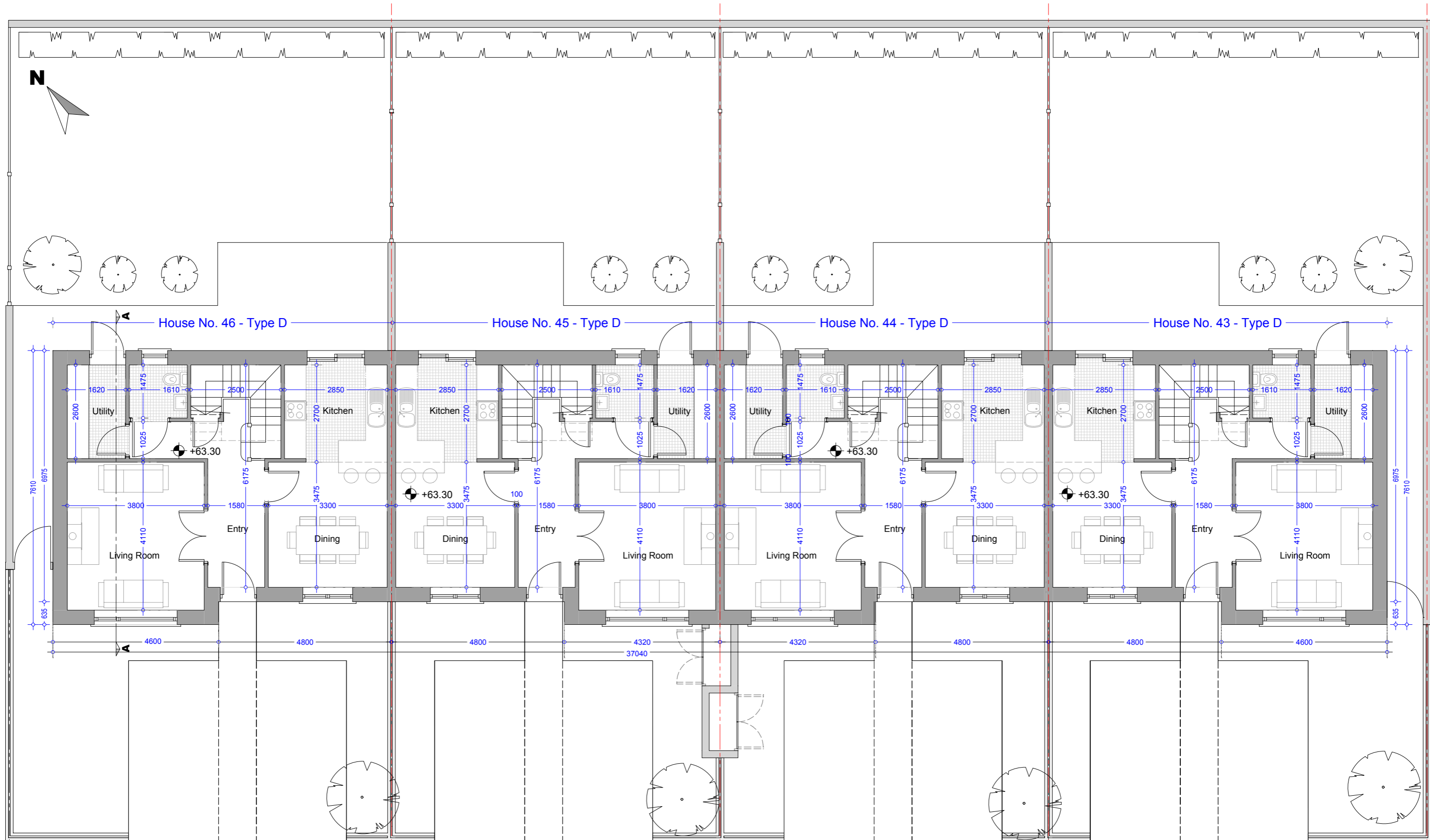
Ground Floor Plan - House D - 3Bed End of Terrace Area = 57.24 m2 / 616.13 sqf
