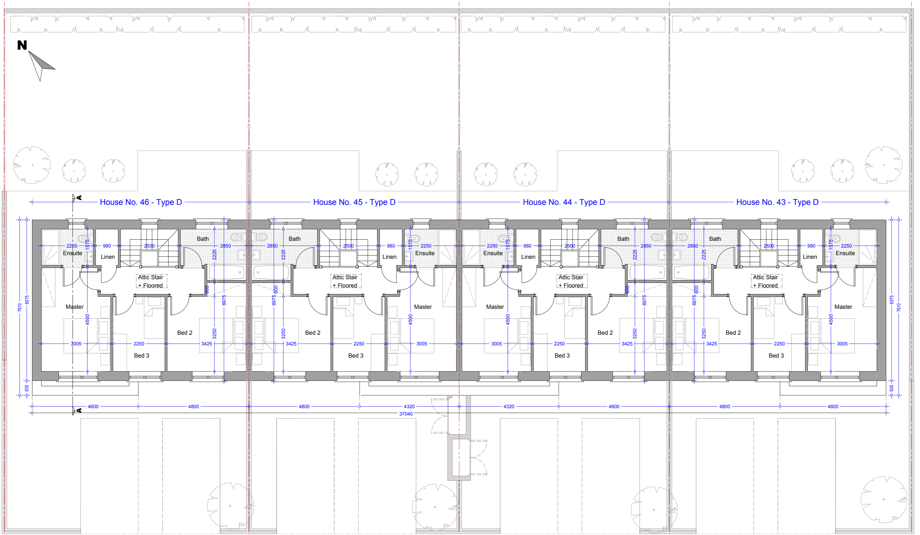
First Floor Plan - House D - 3Bed End of Terrace Area = 54.83 m2 / 590.18 sqf
