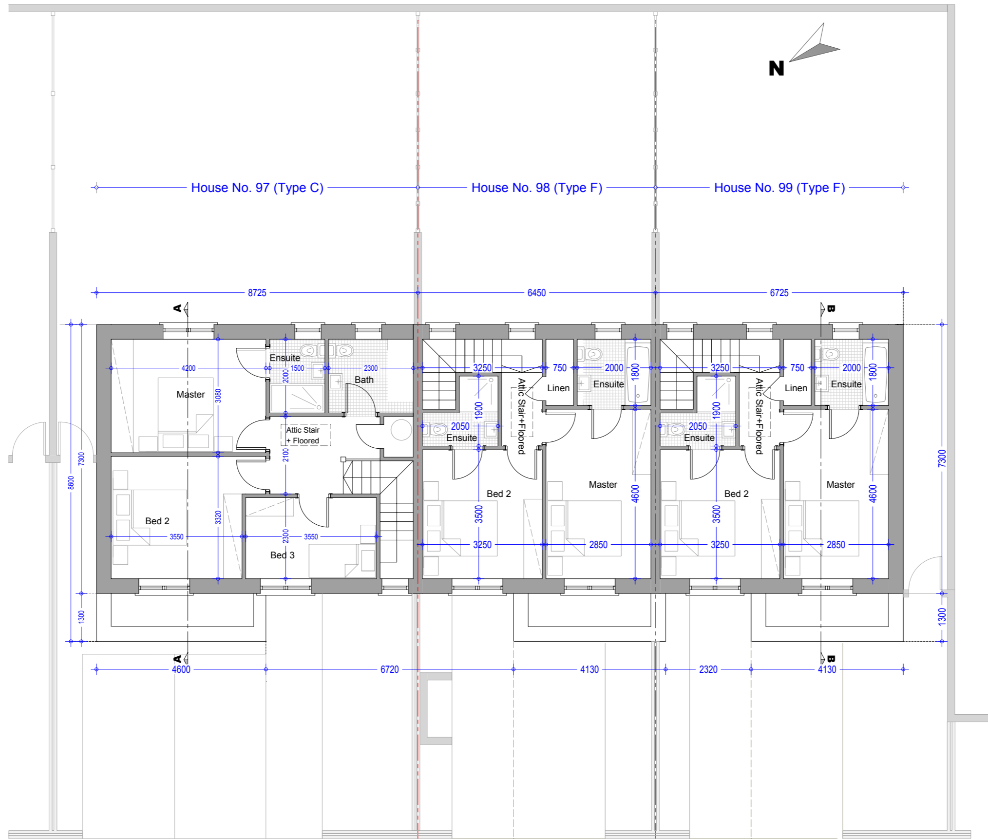
First Floor Plan - House C Area = 53.30 m 2 / 573.72 sqf
