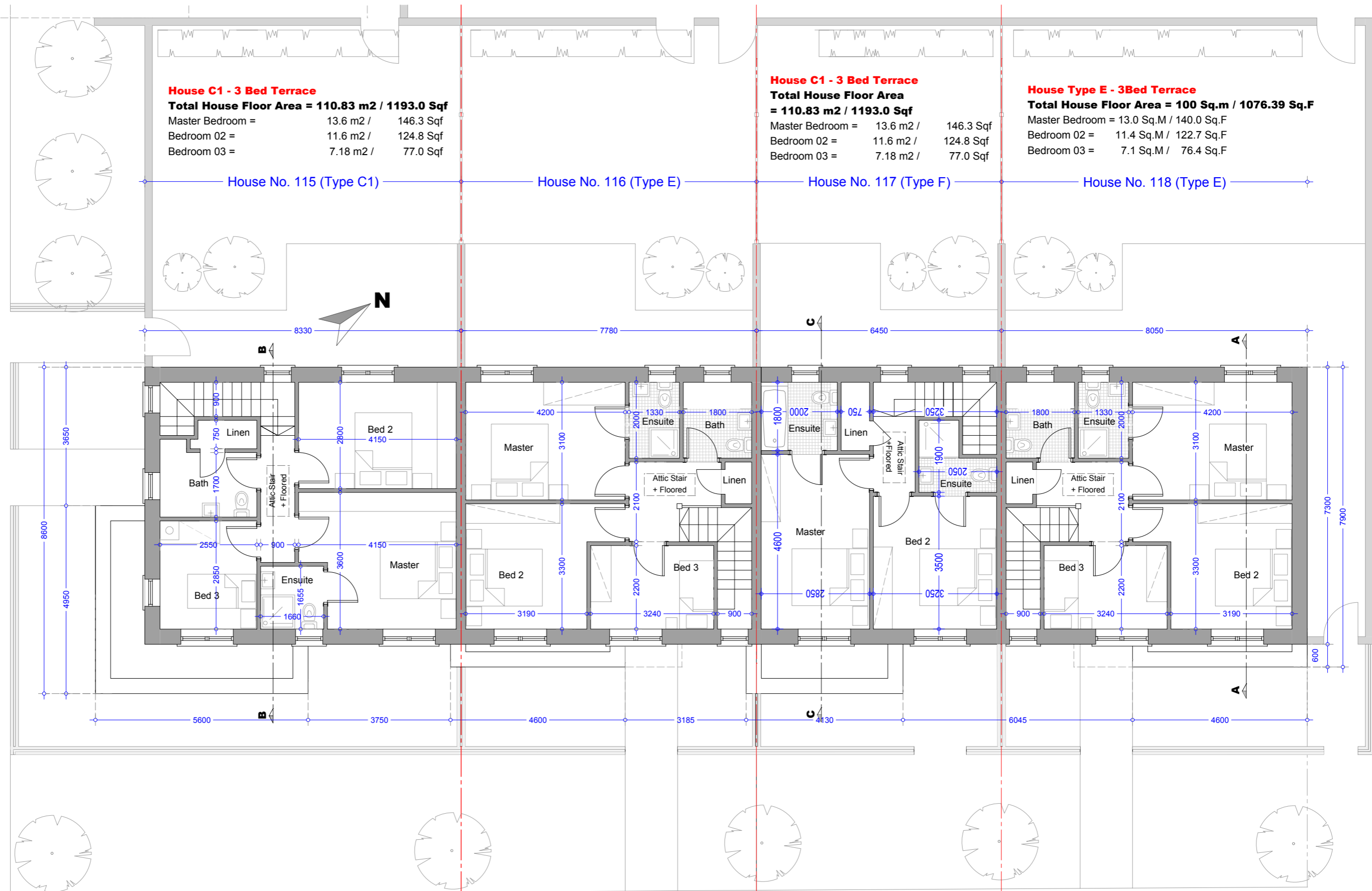
First Floor Plan - House C1 - 3Bed End of Terrace Area = 50.69m2 / 545.62 sqf
