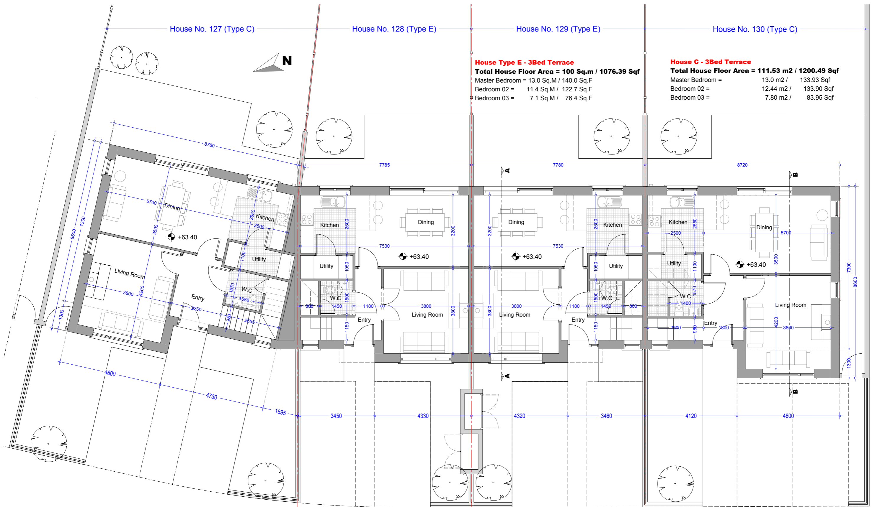
Ground Floor Plan - House E - 3Bed Mid Terrace Area = 51.22 m2 / 551.33 sqf
