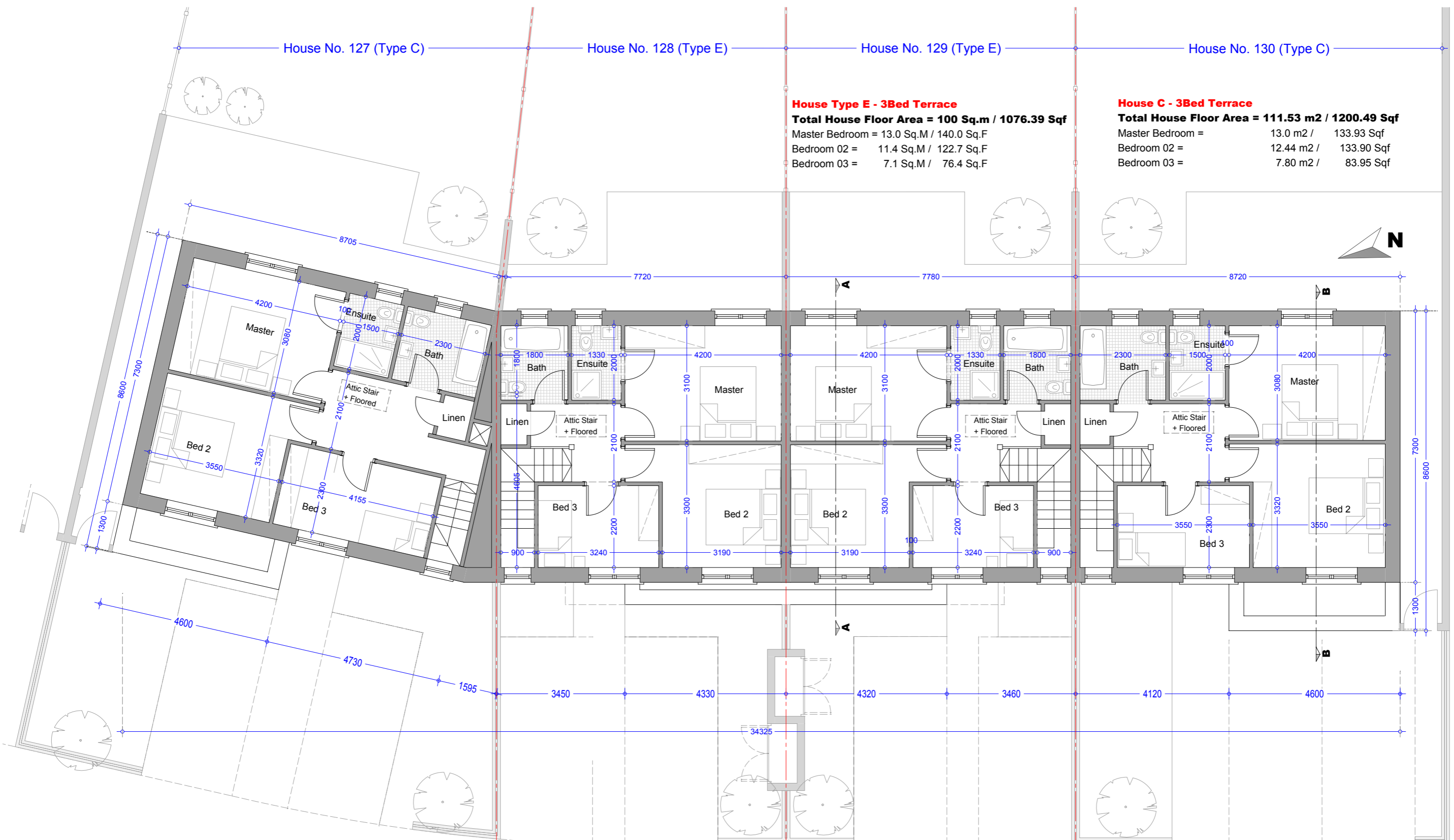
First Floor Plan - House Type C - 3Bed End of Terrace Area = 53.29 m2 / 573.61 Sqf
