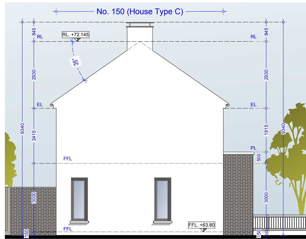
Side Elevation 02 - House Type C (End of Terrace)
