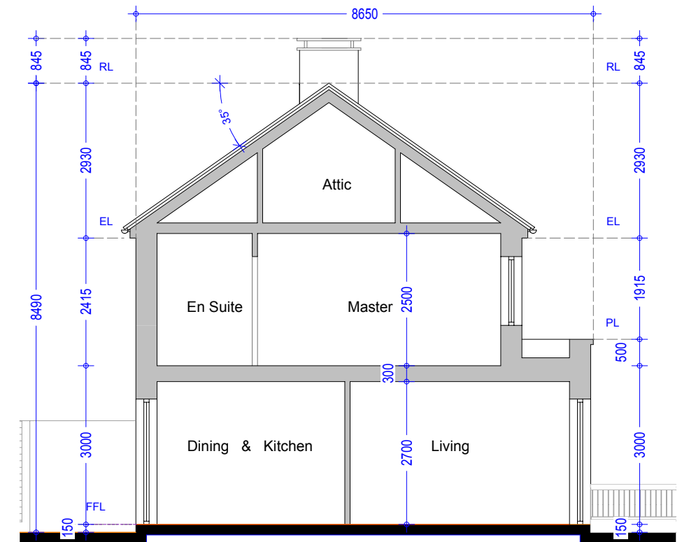
Section CC - House No. 117 - Type F
