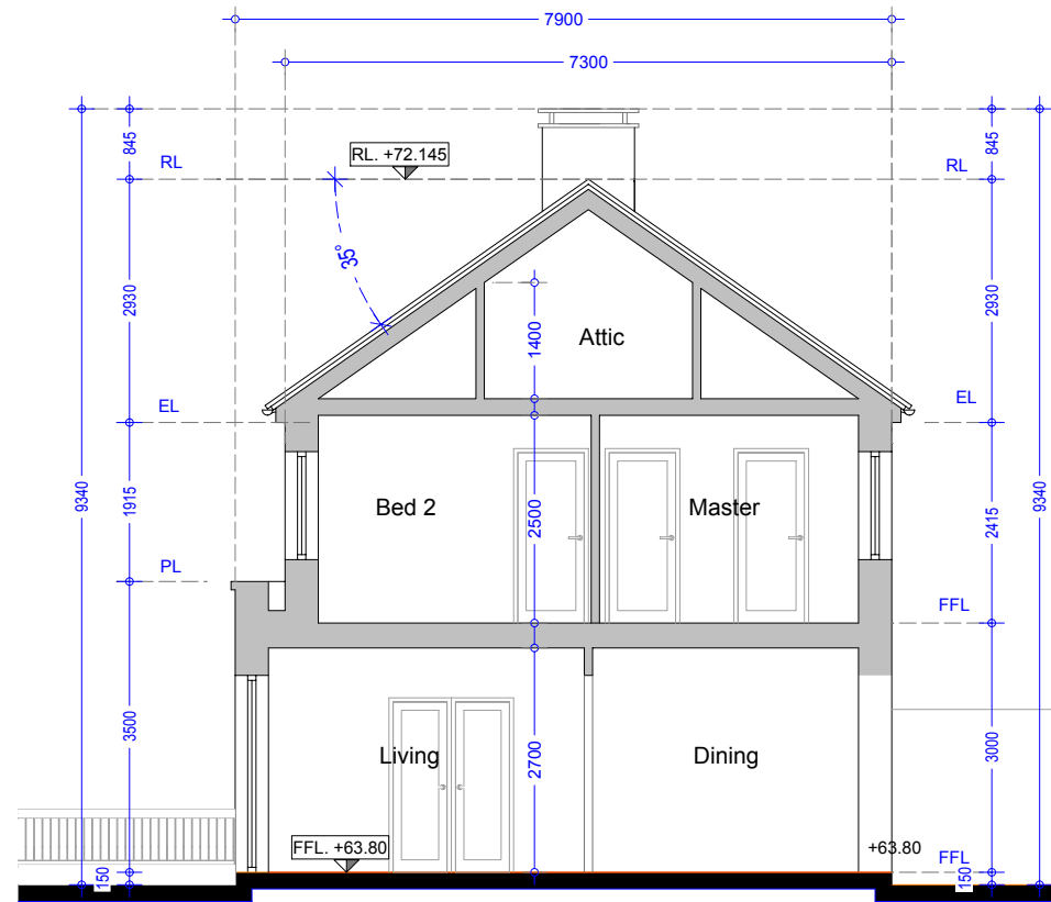
Section AA - House No. 152 - Type E
