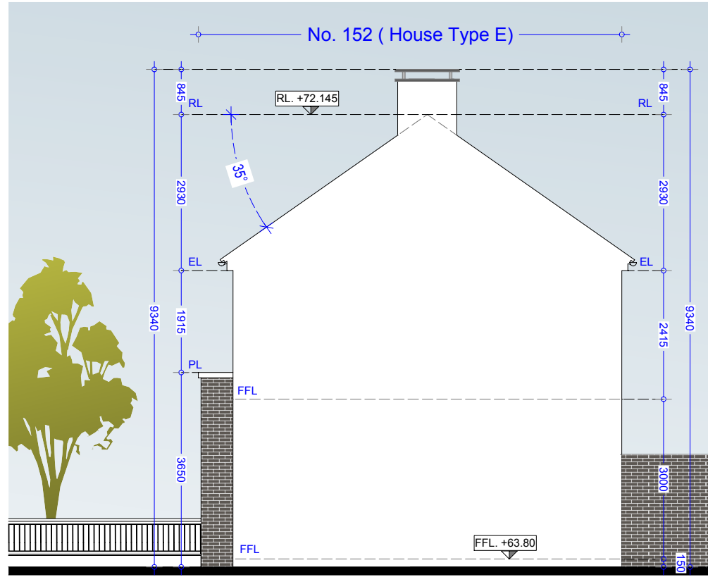
Side Elevation 01 - House Type E (End of Terrace)
