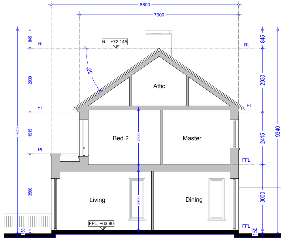
Section BB - House No. 150 - Type C
