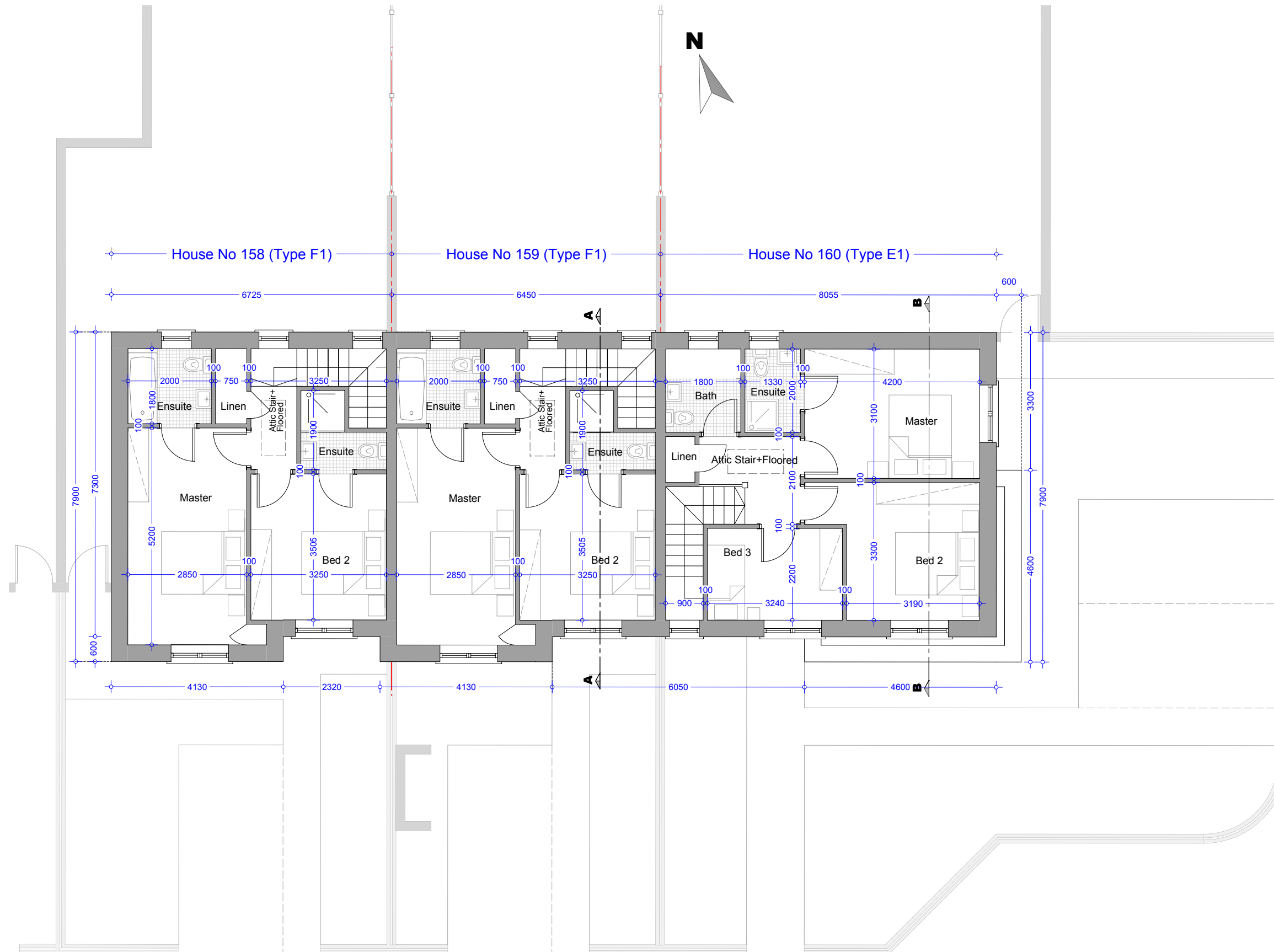
First Floor Plan - House F1 - 2Bed Area = 42.30 m 2 / 455.31 sqf
