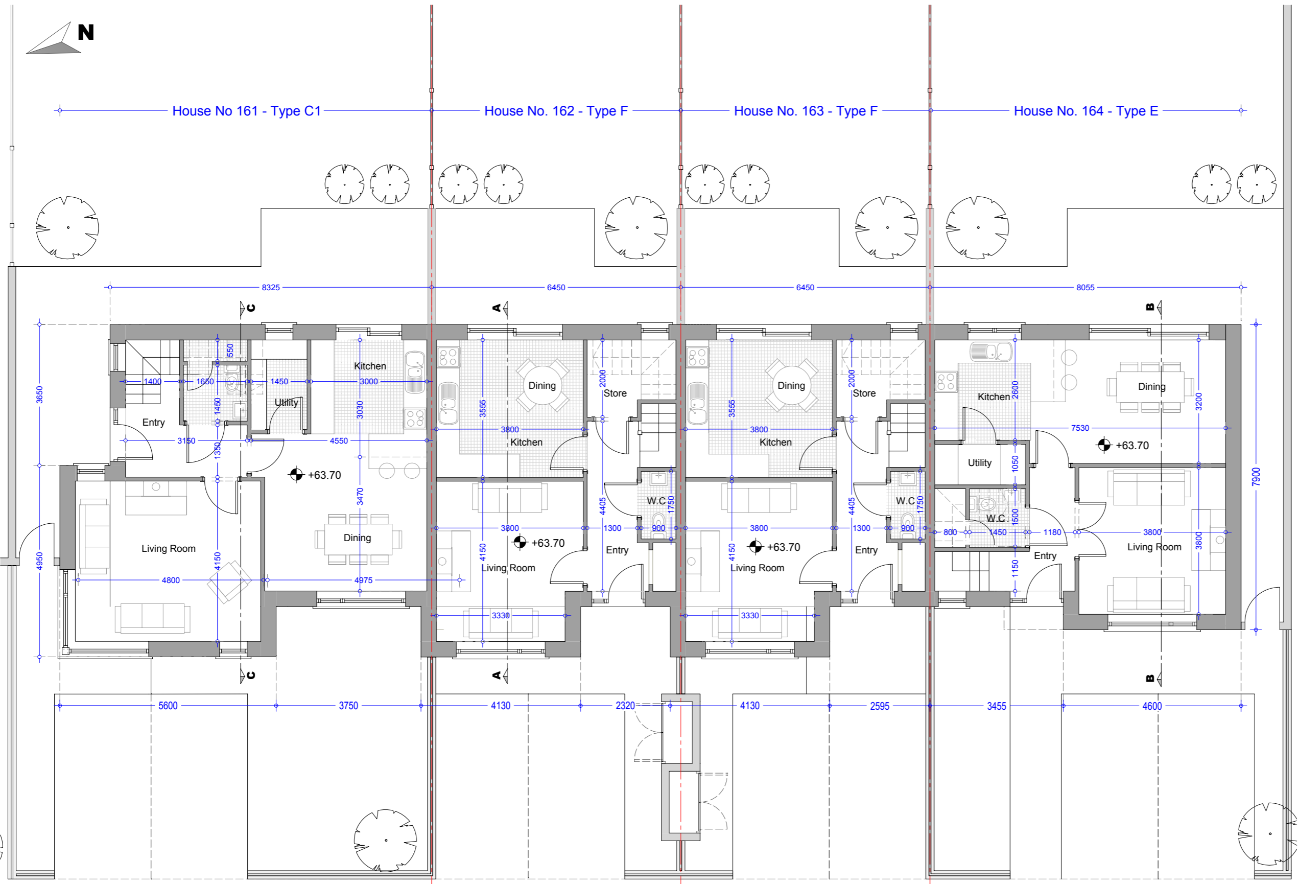
Ground Floor Plan - House C1 - 3Bed End of Terrace Area = 60.63 m2 / 652.62 sqf
