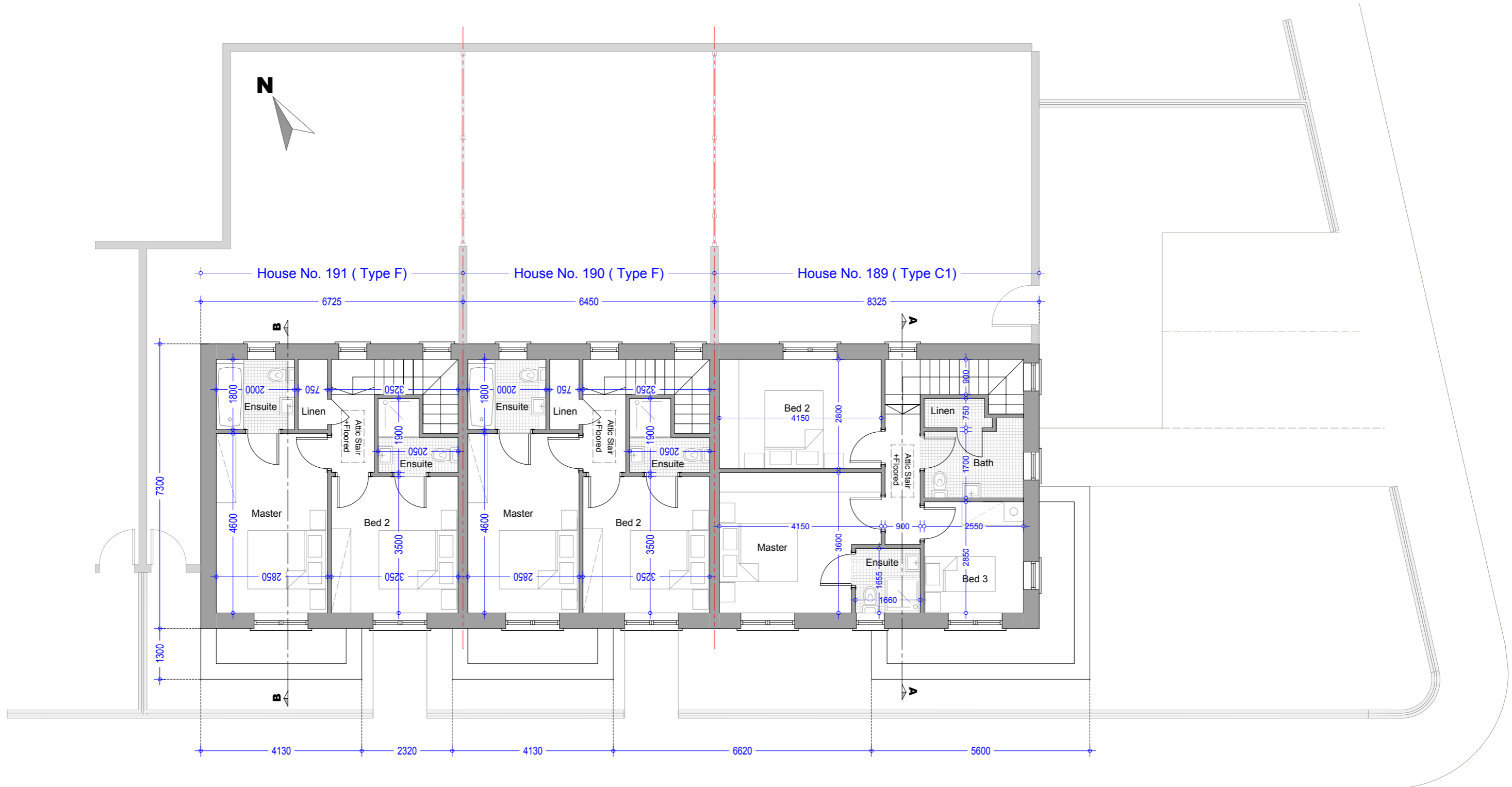
First Floor Plan - House F Area = 40.30 m 2 / 433.79 sqf
