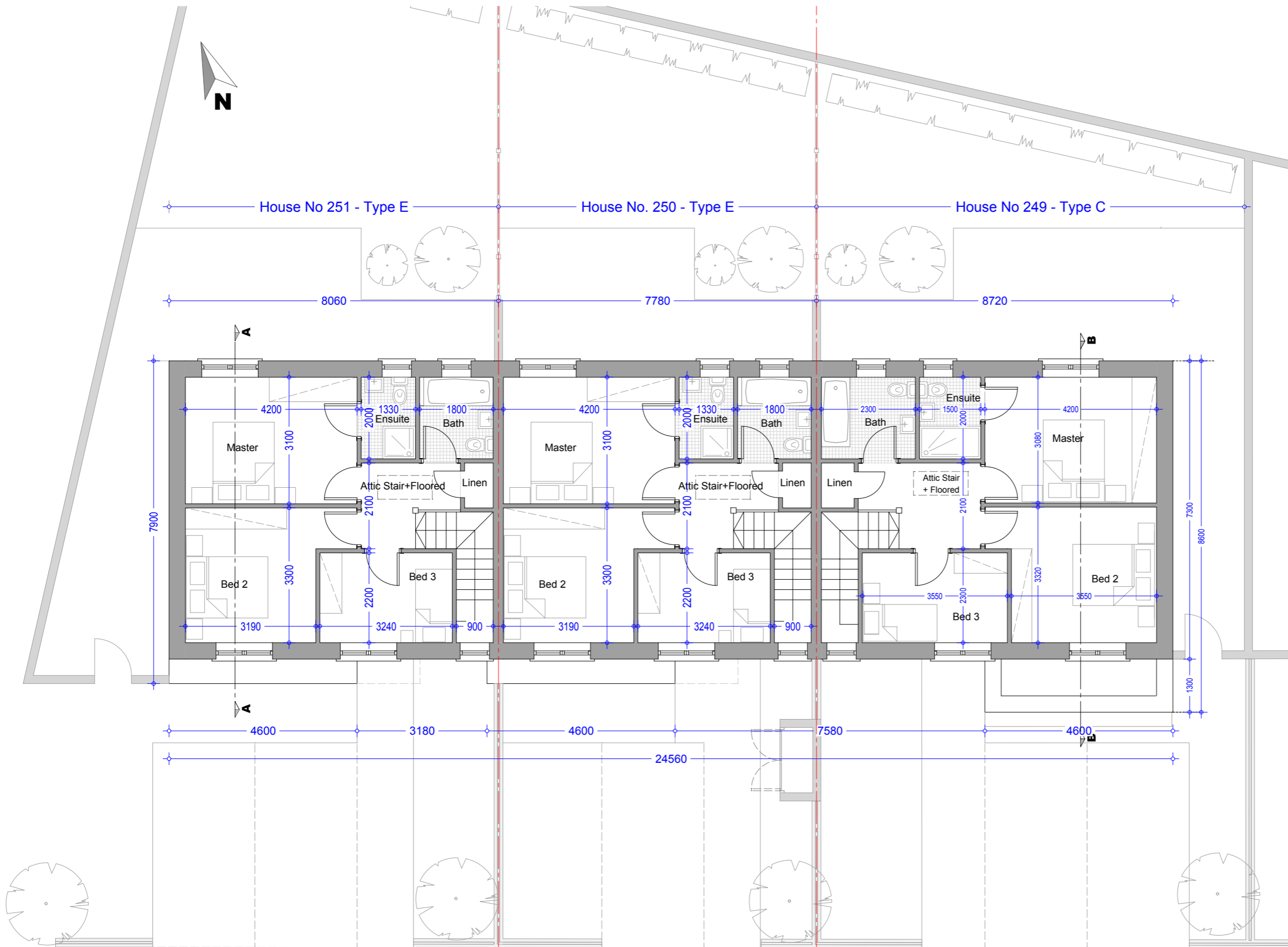
First Floor Plan - House E - 3Bed End of Terrace Area = 48.94 m 2 / 526.79 sqf
