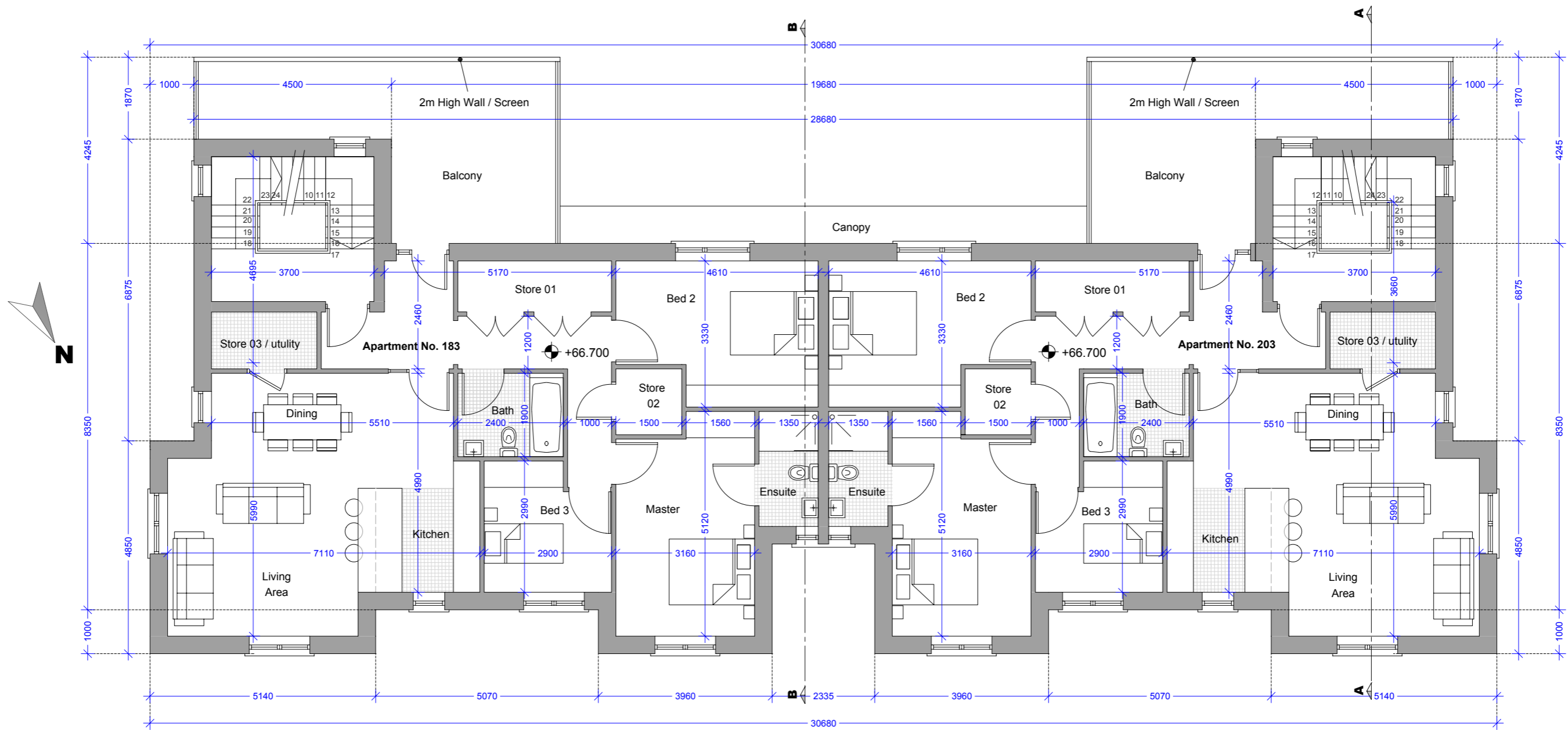
First Floor Plan - 3Bed Apartment - No. 183 (Type G) Area = 108.10 m 2 / 1163.57 Sqf Total First Floor Area = 217.65 m 2 / 2342.76 Sqf
