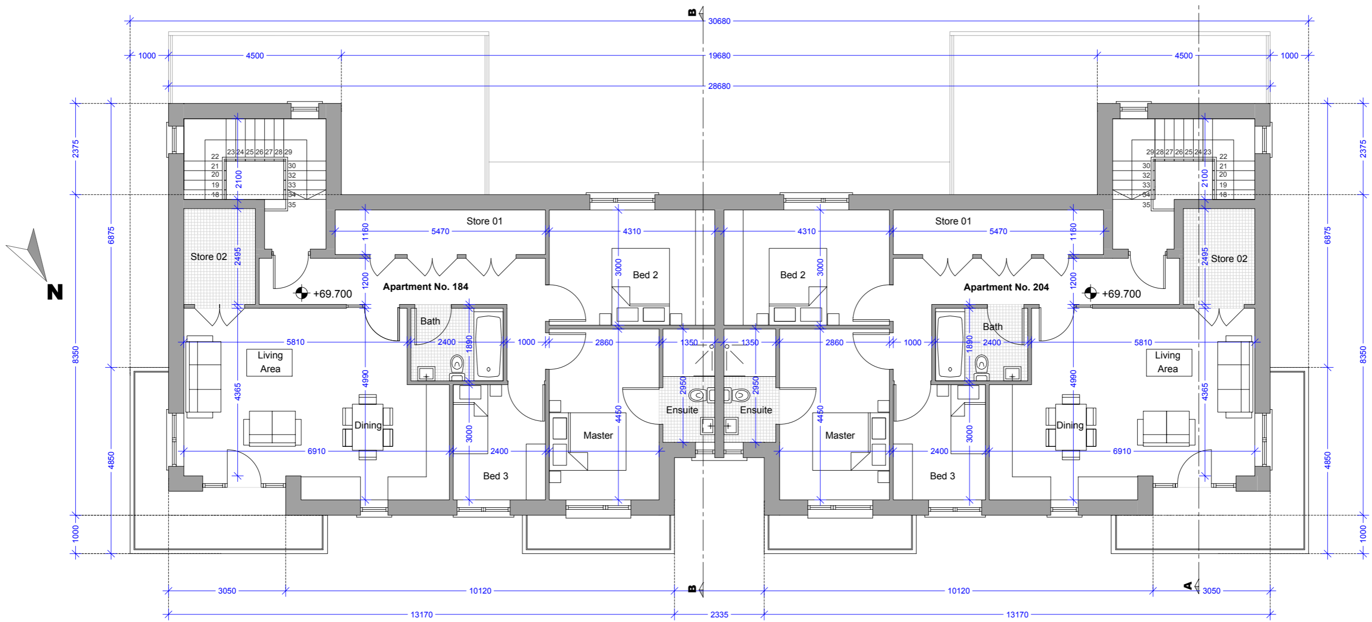
Second Floor Plan - Apartment No. 203 (Type G1) Area = 97.70 m 2 / 1051.63 Sqf Total Second Floor Area = 219.5 m 2 / 2362.7 Sqf
