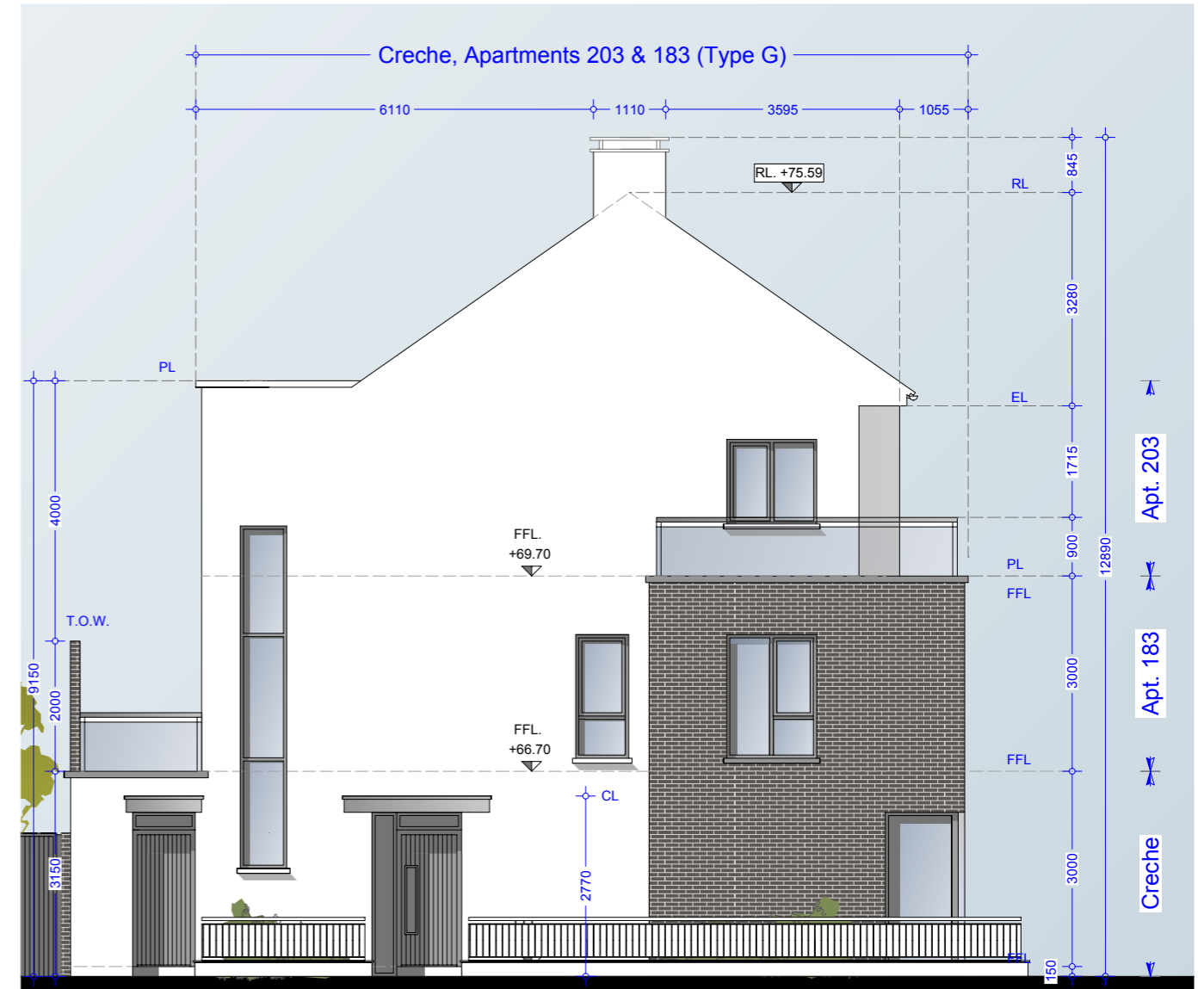
Side Elevation 02 H-Type G - Creche/Apartments
