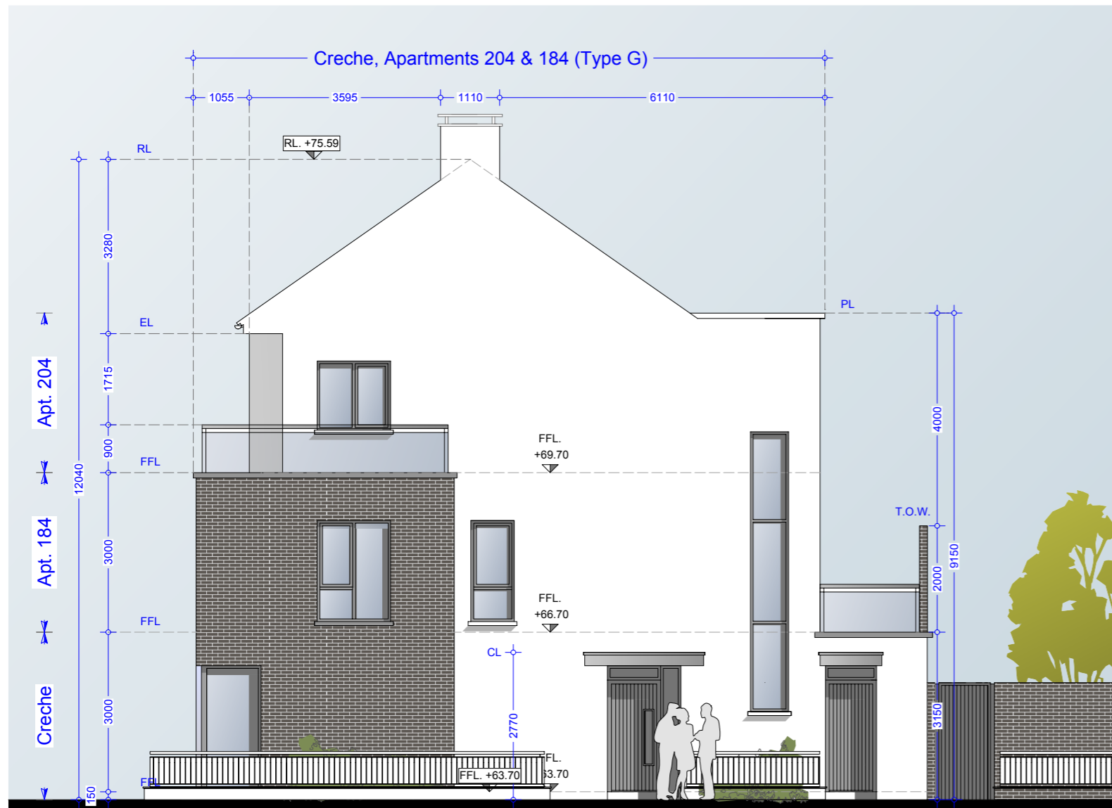
Side Elevation 01 H-Type G - Creche/Apartments
