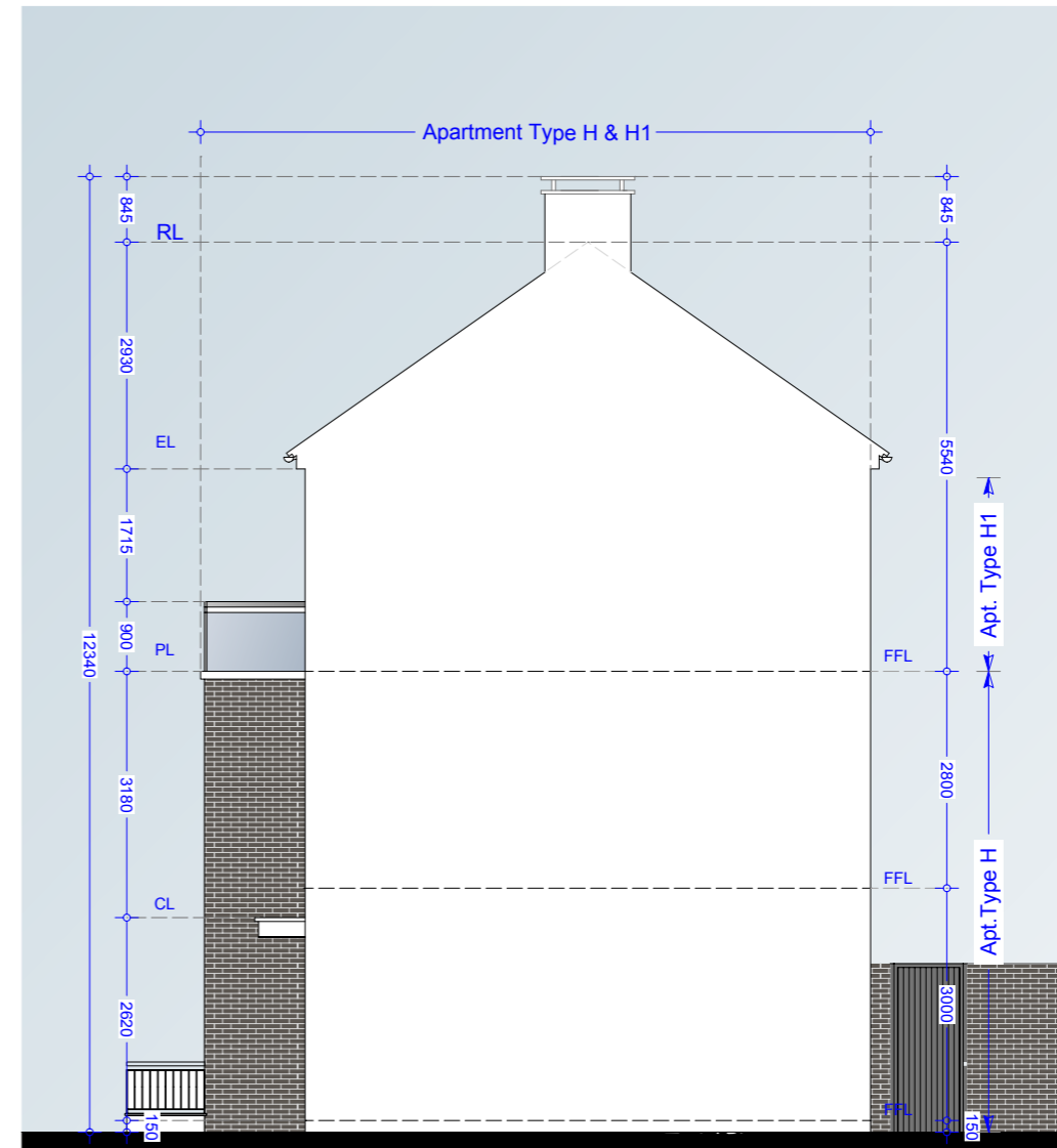
Side Elevation 02 (Mid Street) - Apartment Types H & H1
