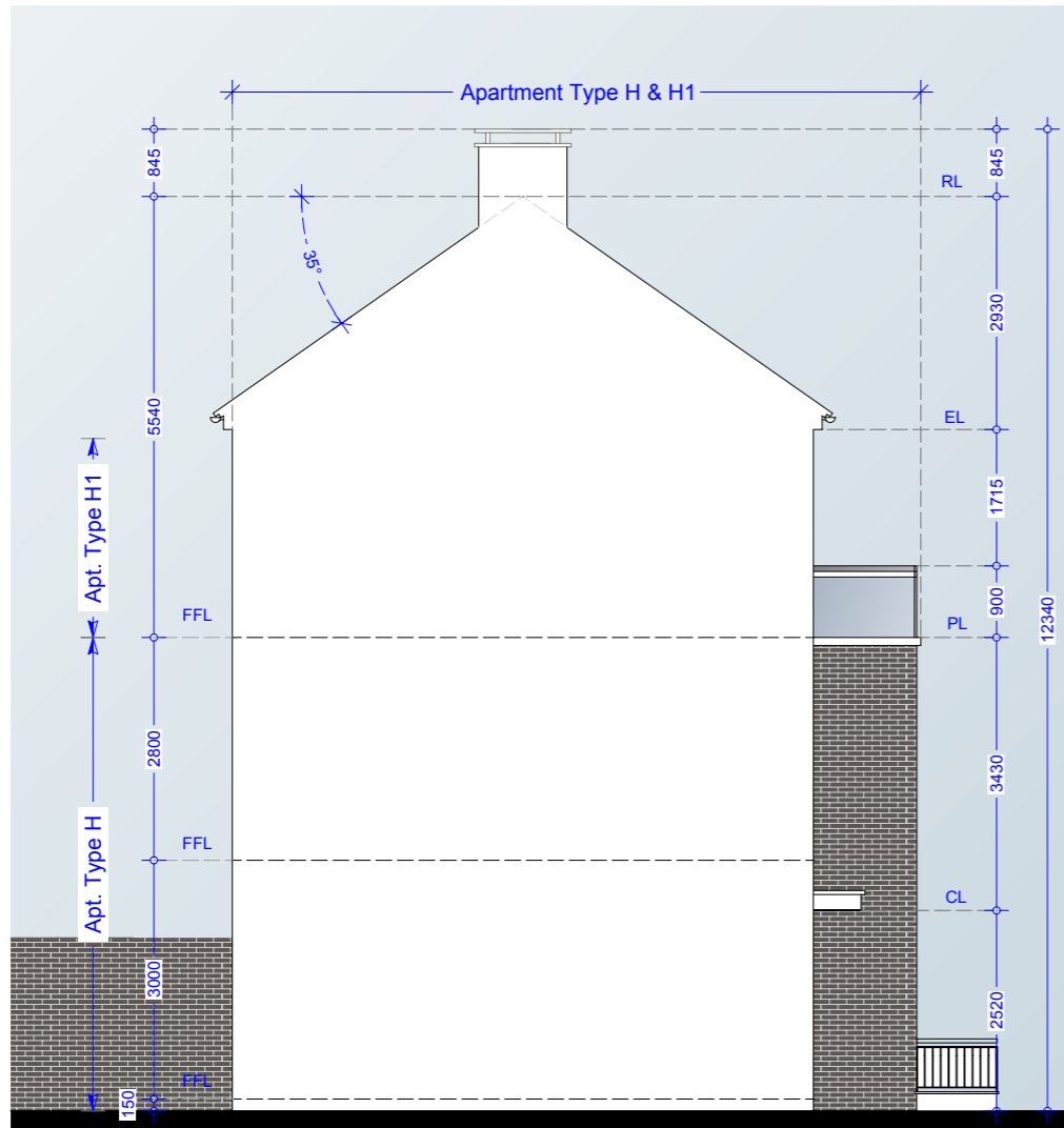
Side Elevation 01 (Mid Street) - Apartment Types H & H1
