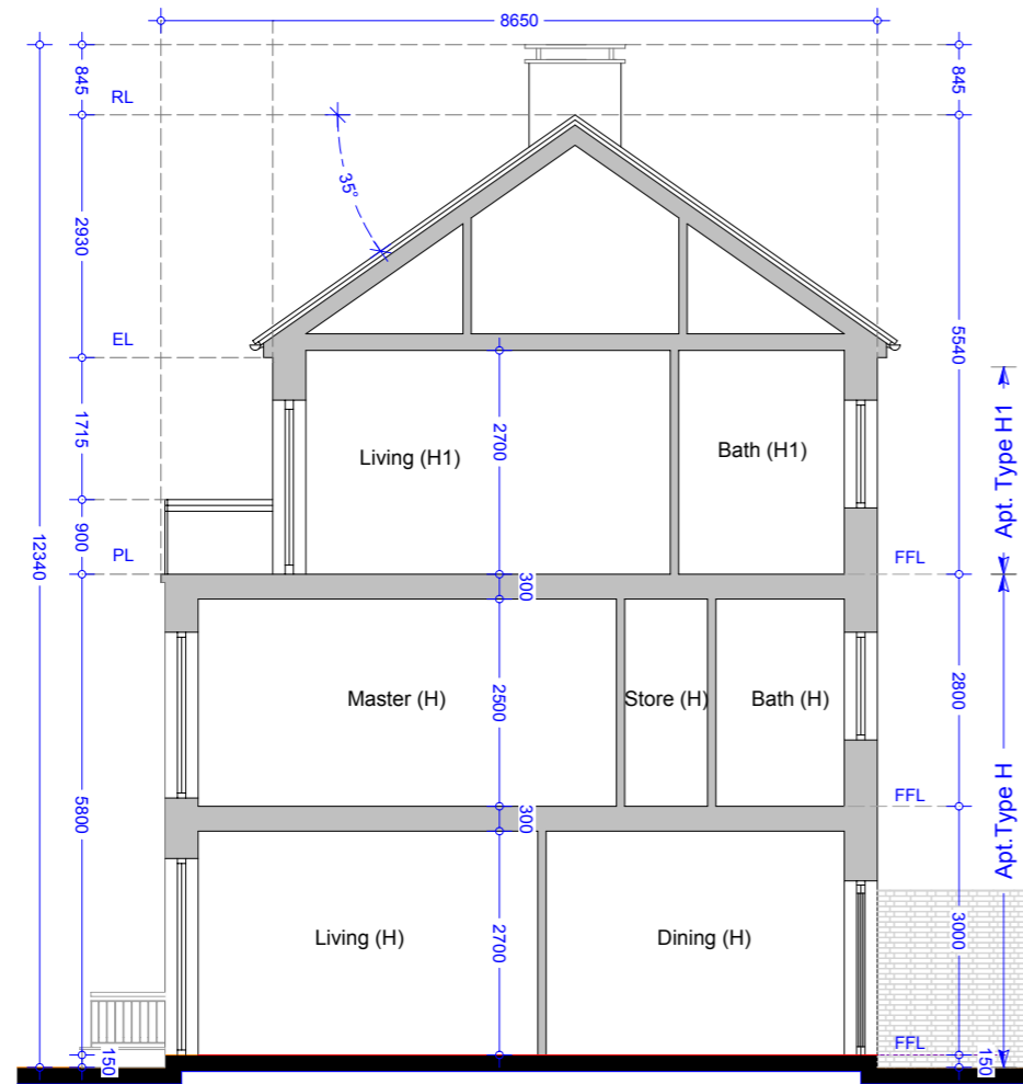
Section A-A - Apartment Types H & H1
