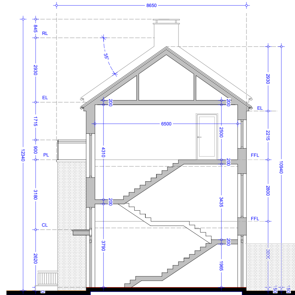
Section B-B - Apartment Types H & H1
