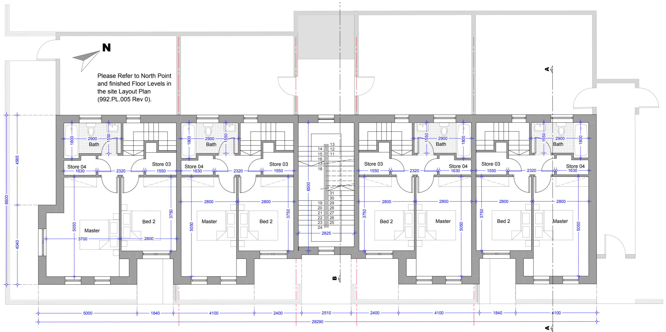
First Floor Plan 2 Bed Duplex Apartment H2 First Floor Area = 43.60 m 2 / 469.31 sqf
