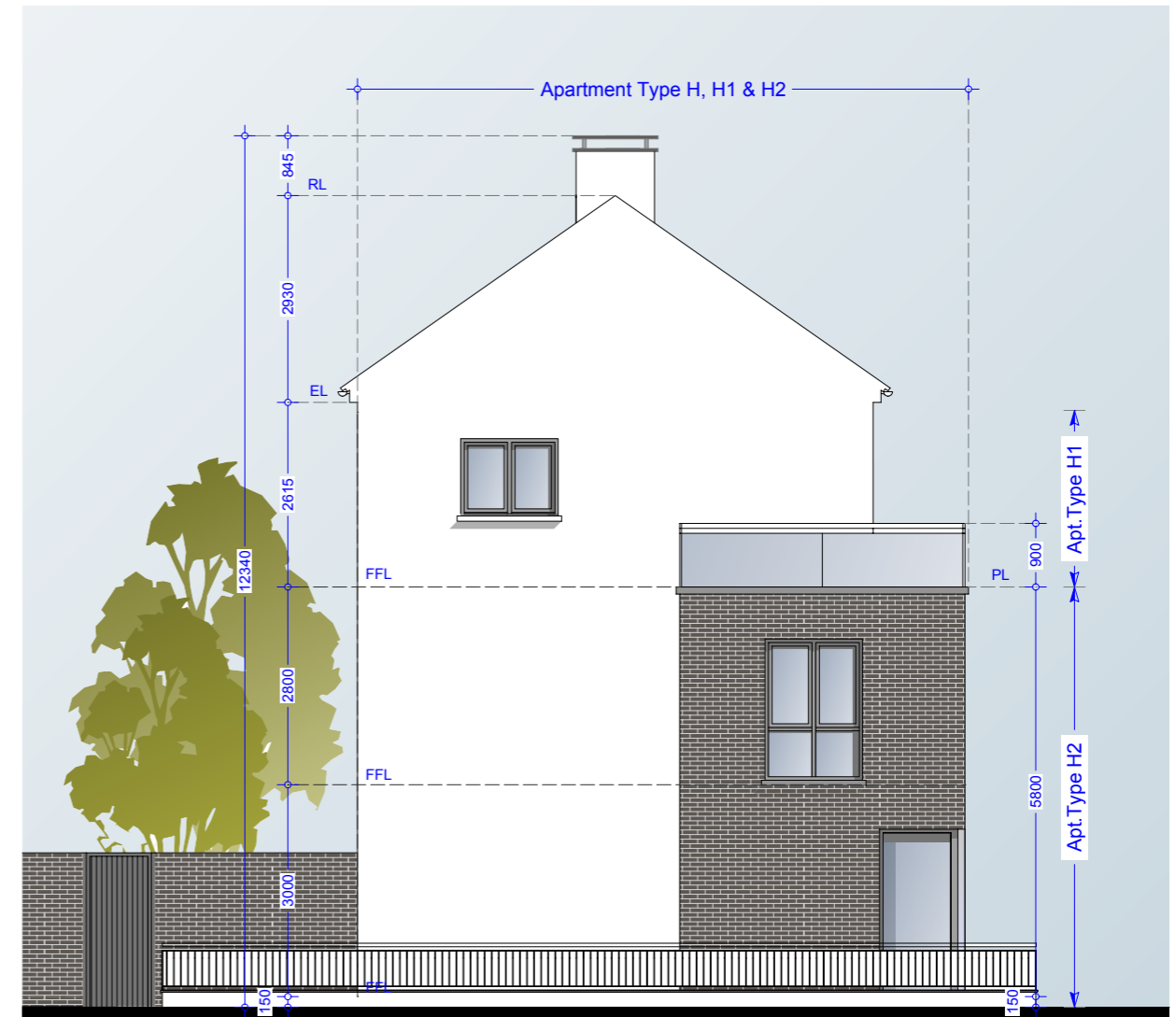
Side Elevation 01 - Apartment Types H, H1 & H2
