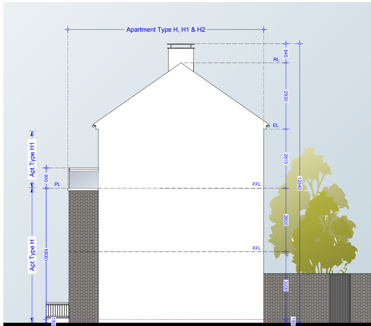
Side Elevation 02 (Mid Street) - Apartment Types H, H1 & H2
