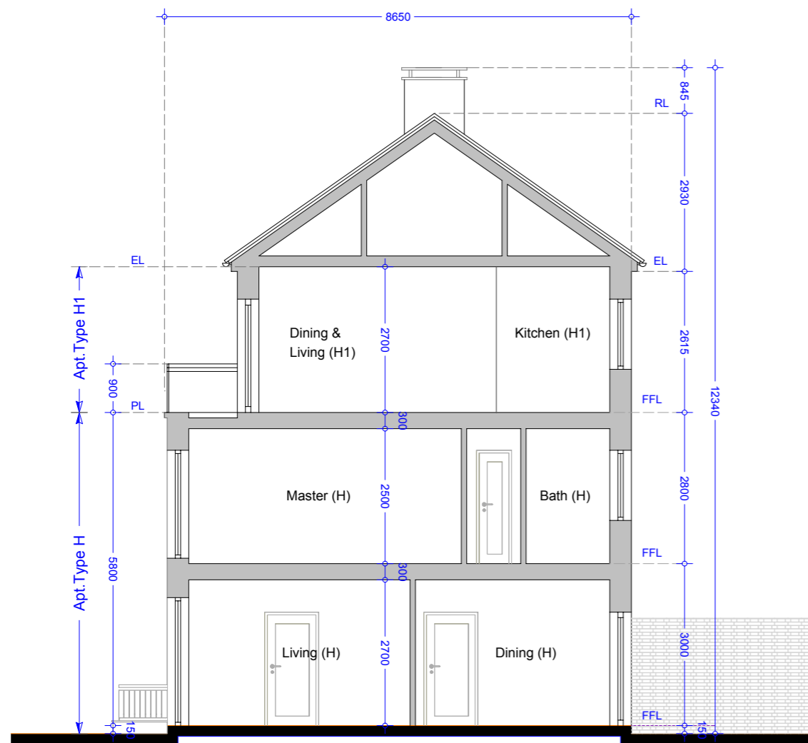
Section AA - Apartment Types H, H1 & H2
