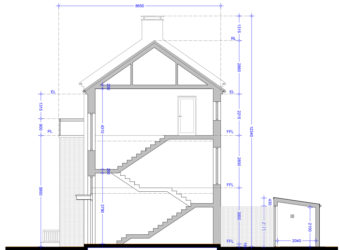
Section BB - Apartment Types H, H1 & H2
