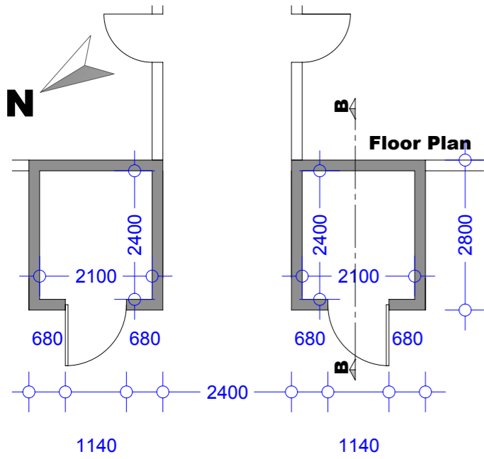
Bin/Bike Store For Apartments 26 & 27
