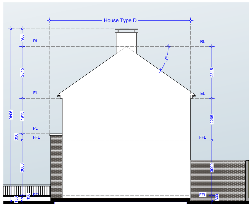
Side Elevation02 - House Type D (Mid Street)
