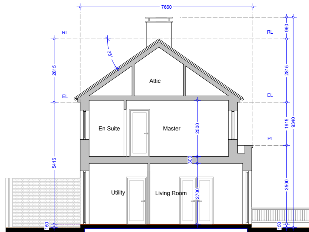
Section AA - House Type D (Mid Street)
