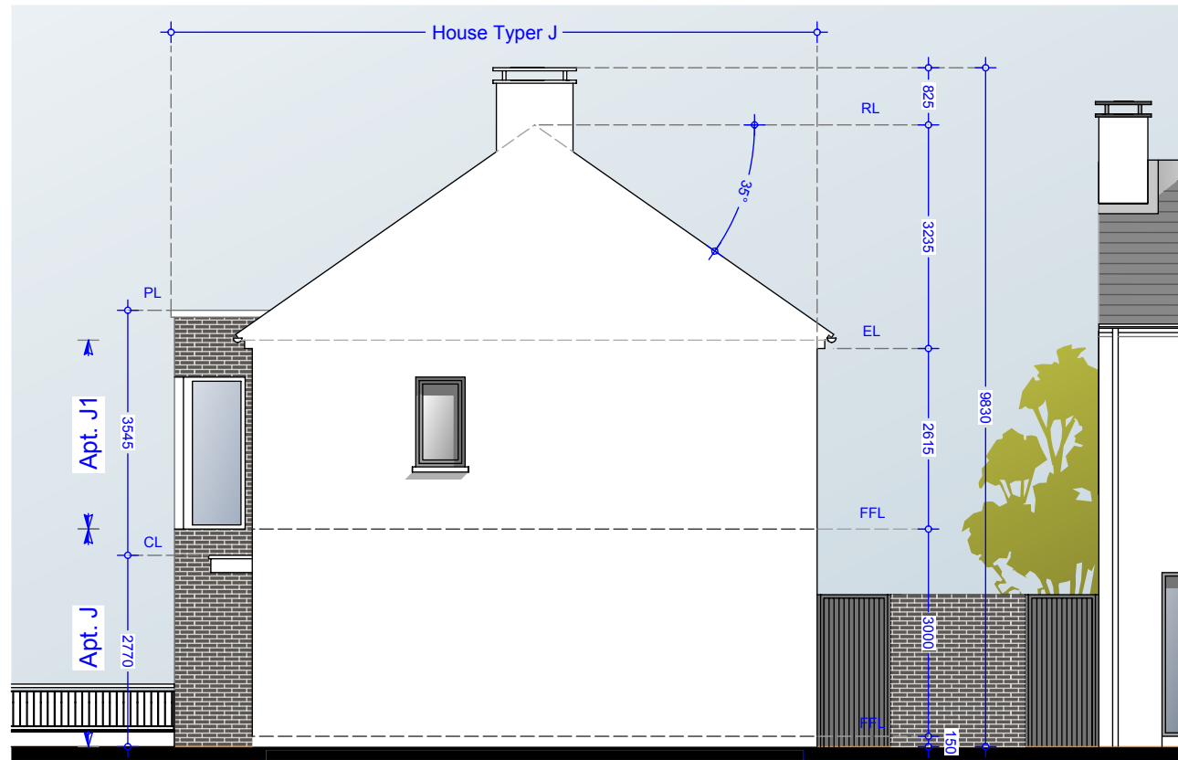
Side Elevation 02 - House Type J & J1
