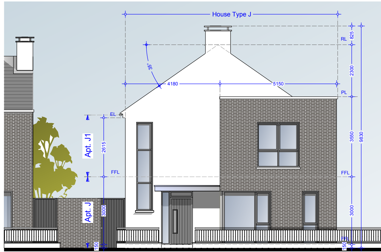
Side Elevation 01 - House Type J & J1 - (First Floor Entrance)
