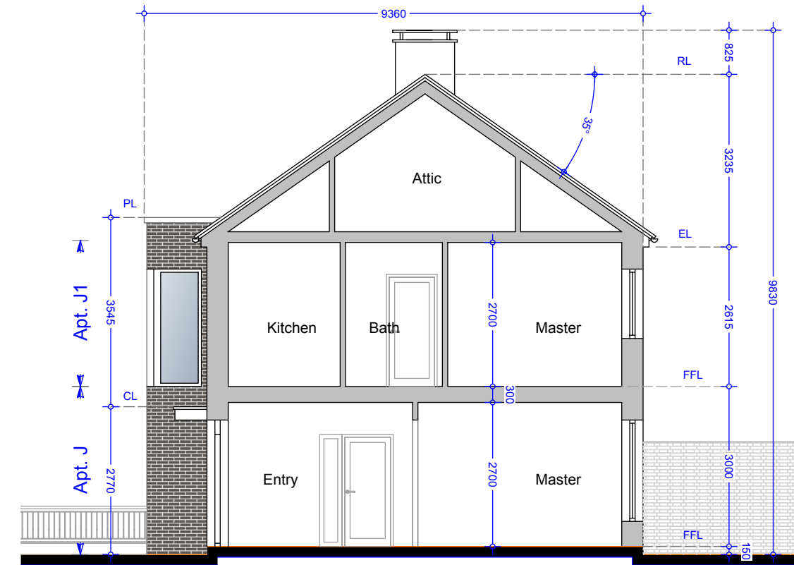
Section A-A - House Type J & J1
