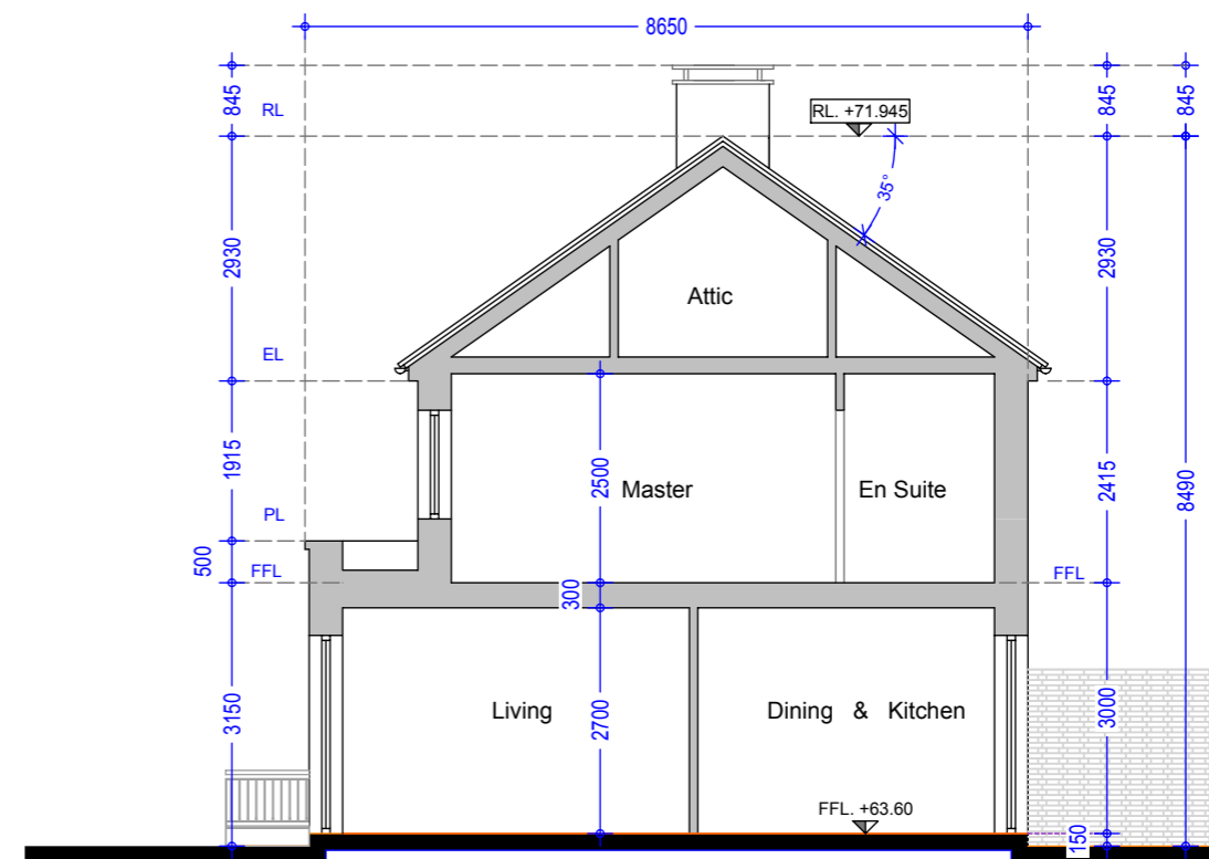
Section B-B - House No. 191 - Type F
