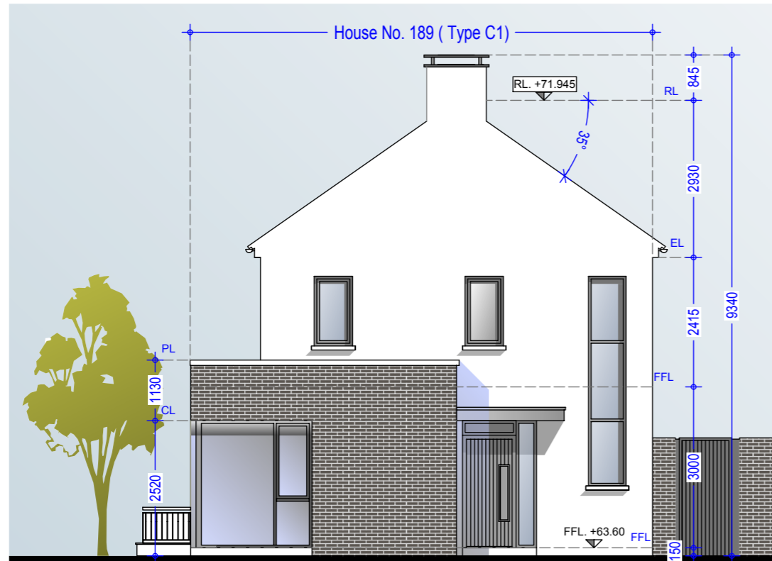
Side Elevation 02 - House Type C1
