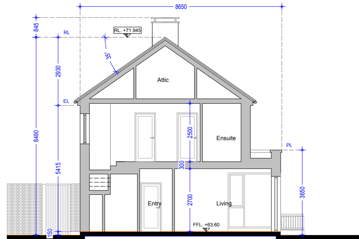
Section A-A - House No. 189 - Type C1
