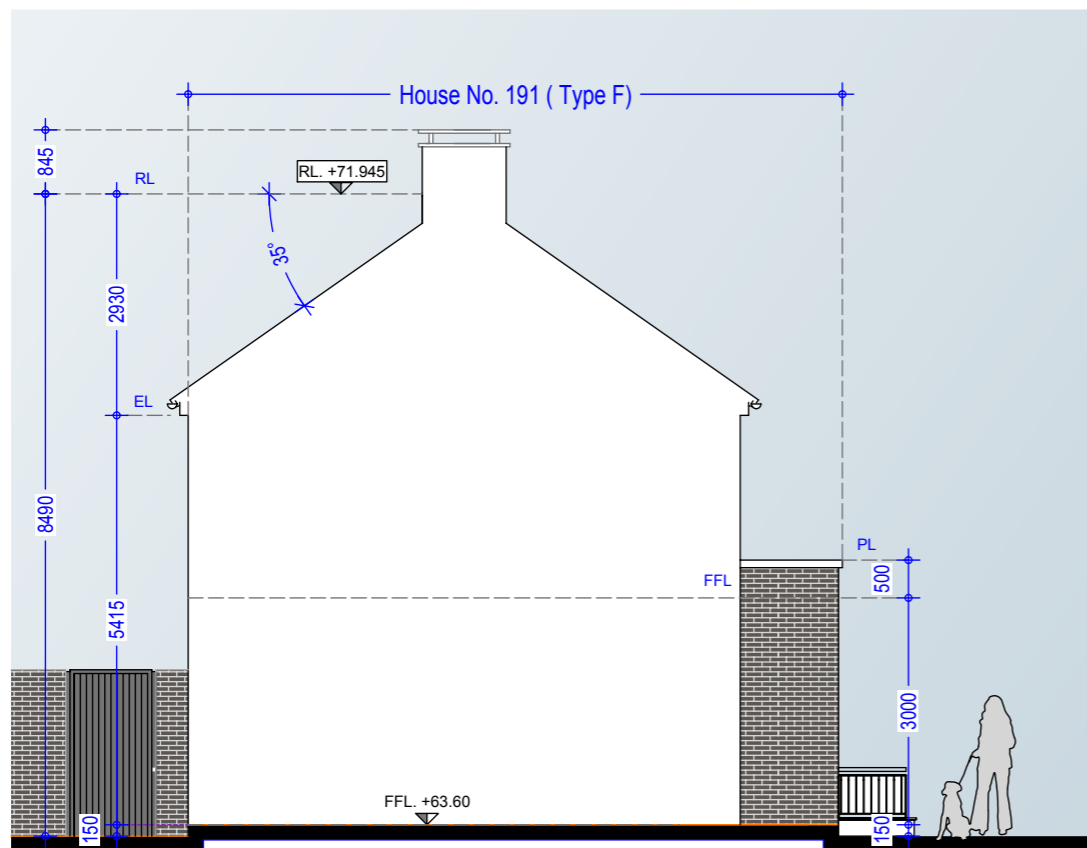
Side Elevation 01 - House Type F
